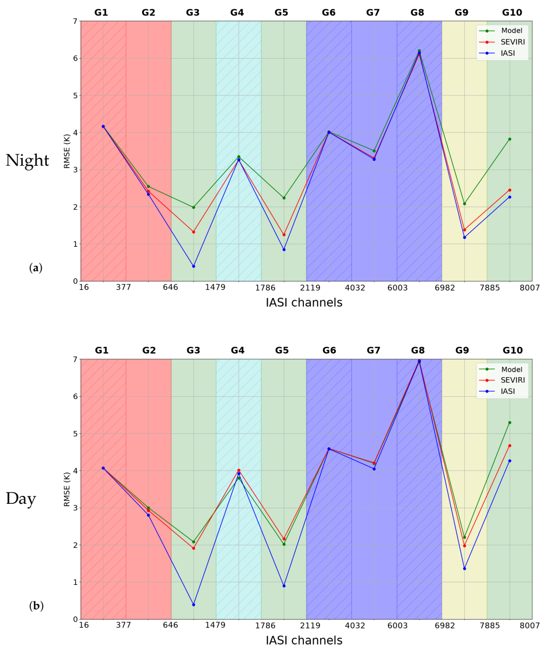
Figure 11. Nighttime (a) and daytime (b) root mean square errors related to simulations of IASI brightness temperatures using model LST (green line), SEVIRI LST (red line) and IASI LST (blue line) of surface (green), Temperature (orange), ozone (cyan), water vapour (blue) and solar (yellow) sensitive channels. Hatched areas of the figure correspond to channels that present very small sensitivity to LST.
