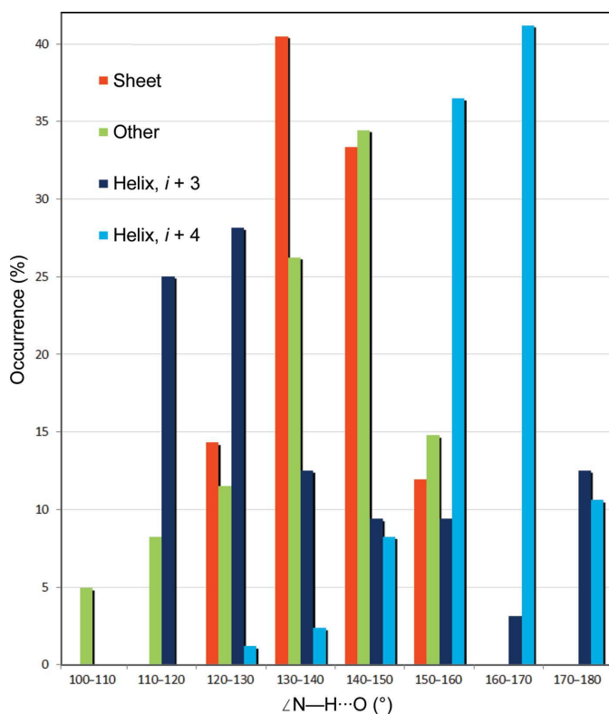
Figure 15 Percentage distribution of \angle \text{N}-\text{H} \cdots \text{O} as found in the \text{C}=\text{O} \cdots \text{H}-\text{N} hydrogen bonds for \alpha -helices, \beta -sheets and ‘other’ parts of the ChOx protein.
