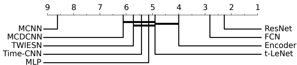
Fig. 10: Critical difference diagram showing pairwise statistical difference comparison of nine deep learning classifiers on both univariate and multivariate time series classification archives.
