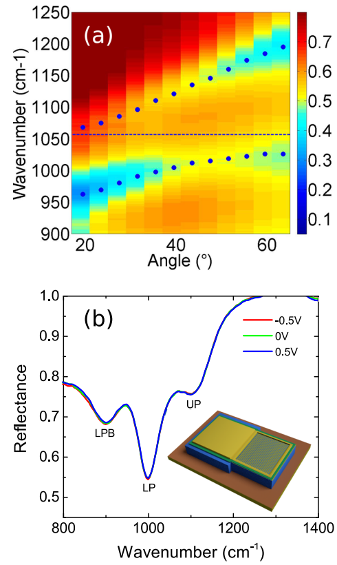
FIG. 3. (a) Room temperature reflectivity dispersion from 17^\circ to 65^\circ of a 2.5 \times 2.5\text{ mm}^2 polaritonic cavity. The grating period is 3.8\text{ }\mu\text{m} and the filling factor is 70%. The blue dots correspond to the RCWA simulation with an ISB transition at 31.7\text{ THz} and a doping of 5.5 \times 10^{11}\text{ cm}^{-2} . (b) Reflectivity spectra at 20^\circ \pm 5^\circ and 78 K acquired with a FTIR microscope (resolution is 8\text{ cm}^{-1} ) on a 150 \times 150\text{ }\mu\text{m}^2 , 3.5\text{ }\mu\text{m} period and 80% filling factor SC-QWIP under different biases. The upper and lower polaritonic branches are indicated as UP and LP, while LPB indicates the Bragg-folded lower photonic branch. 17 There is no change in absorption as a function of the applied voltage. The sample temperature is 78 K. The inset shows the schematic of a SC-QWIP device: active region (blue), SiN insulator (green), gold top contact (yellow) and ohmic PdGe bottom contact (dark orange).
