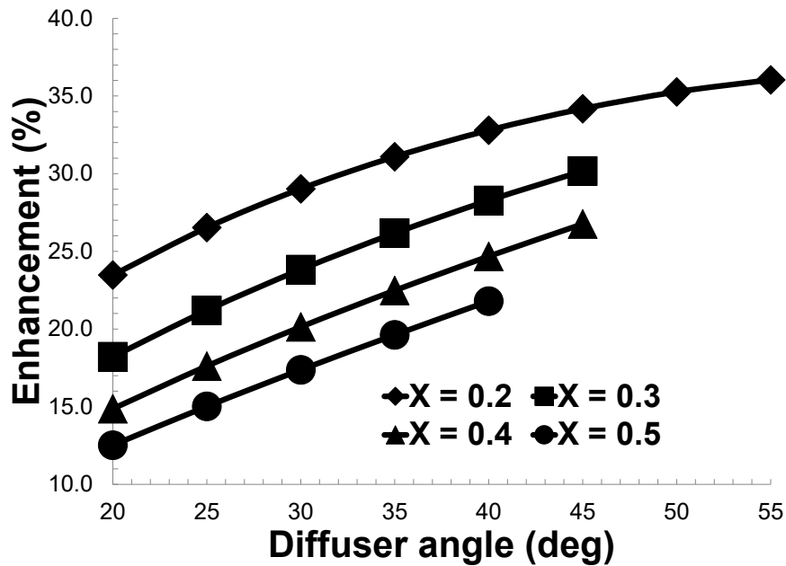
Figure 7: Variation of the thermal performance enhancement in function of the diffuser angle for different X .
