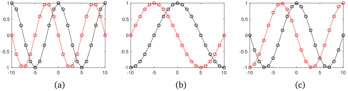
Figure 7: In (a) and (b): two atoms a(z) = (a(z)_m)_{m=-M}^M and a(z') = (a(z')_m)_{m=-M}^M , respectively, with z = e^{i2\pi/10} , z' = e^{i2\pi/20} , M = 10 ; the index m is in abscissa, the real and imaginary parts of the values are in ordinate, with black and red colors, respectively. In (c): the atomic Wasserstein barycenter v \in \mathbb{V} , which minimizes \tilde{d}_{a_2, z}(v)^2 + \tilde{d}_{a_2, z'}(v)^2 ; it turns out that v is the atom a(e^{i3\pi/20}) , whose frequency is the mean of the frequencies of the two given atoms.
