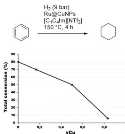
Scheme 5. Conversion as a function of the molar fraction of Cu in bimetallic Ru–Cu NPs for the hydrogenation of benzene. Reproduced from reference [86] with the permission of Springer.
