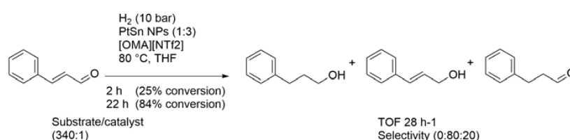
Scheme 4. PdSn-based BMNPs stabilized by [\text{OMA}][\text{NTf}_2] as the catalyst for the hydrogenation of cinnamaldehyde [85].
