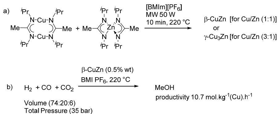
Scheme 7. (a) Synthesis of CuZn alloys in [C_1C_4Im][PF_6] by the decomposition of amidinate precursors under microwave activation. (b) Production of methanol catalyzed by the \beta -CuZn alloy [90].
