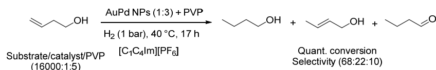
Scheme 3. AuPd BMNPs applied in the hydrogenation of 3-buten-1-ol [79].
