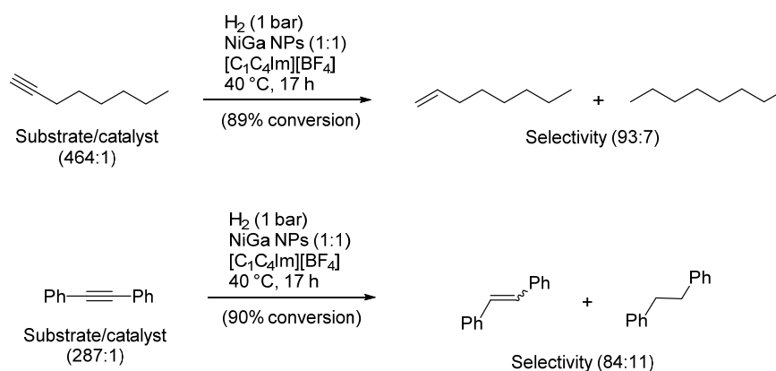
Scheme 8. Semihydrogenation of alkynes catalyzed by NiGa BMNPs [91].
