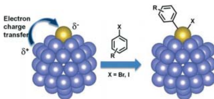
Figure 2. Electronic transfer from Ni (blue) to Pd (yellow) and the oxidative addition of aryl halides on Pd atoms. Reproduced from reference [24] with permission of The Royal Society of Chemistry.
