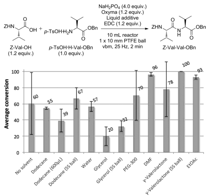
Figure 1. Liquid additive influence on average conversion and chemical homogeneity during the mechanochemistry of Z-Val-Val-OBn.
