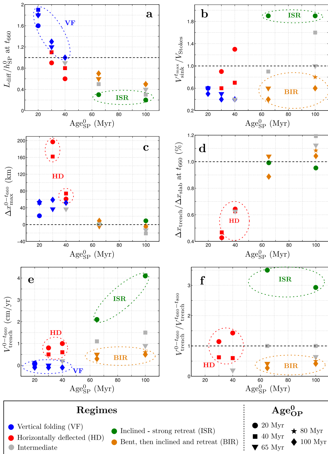
Figure 7. Evolution of diagnostic outputs as a function of initial subducting plate age Age_{SP}^0 for all simulations with \Delta\mu=30 : (a) L_{diff}/h_{SP}^0 at t_{660} , (b) V_{sink}^{max}/V_{Stokes} , (c) \Delta x_{max}^{0-t_{660}} (km), (d) \Delta x_{trench}/\Delta x_{slab} at t_{660} , (e) V_{trench}^{0-t_{660}} , and (f) V_{trench}^{0-t_{660}}/V_{trench}^{t_{660}-t_{800}} . Initial overriding plate ages and subduction regimes are labeled by symbols and colors, respectively. VF cases (with quasi-stationary trenches) have been removed for Figures 7d and 7f.
