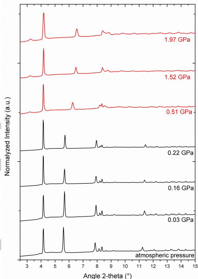
Figure 1. Powder X-ray diffraction patterns ( \lambda = 0.694120 \text{ \AA} ) obtained for the MIL-53(Cr) as a function of the applied pressure at room temperature. Patterns in black line correspond to the monoclinic (S.G. C2/c ) hydrated Narrow Pore form and in red line to the triclinic (S.G. P-1 ) Very Narrow Pore form.
