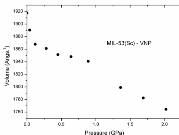
53 54 55 56 57 58 59 60 61 62 63 64 65 Figure 6. Evolution of the pressure-induced unit cell volume of the Very Narrow pore form of MIL-53(Sc).
