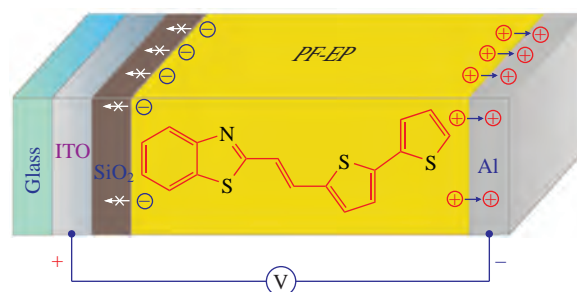
Figure 2 Schematic diagram of MIS-CELIV measurement device.
