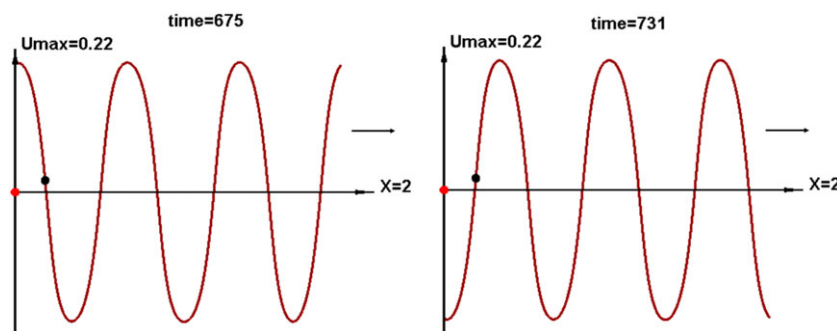
FIGURE 4 Snapshots of the periodic wave. It is a periodic in space solution moving with a constant speed. The function in the right figure can be obtained from the function in the left figure by a shift on half-period [Colour figure can be viewed at wileyonlinelibrary.com ]
