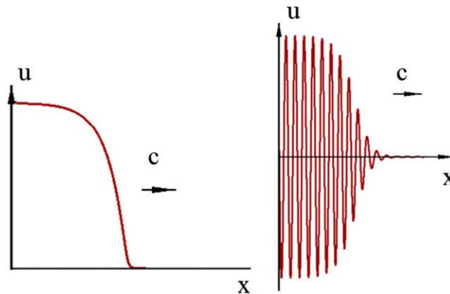
FIGURE 3 Snapshots of a monotone wave (left) and of a wave with a stationary periodic structure behind it (right) [Colour figure can be viewed at wileyonlinelibrary.com ]
