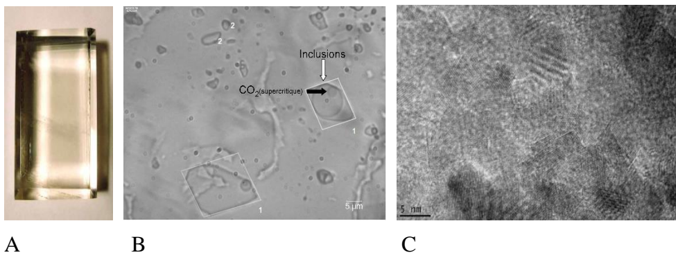
Fig. 1. Macroscopic calcite mono-crystal (A) of optical quality, observed at the micrometre scale (B) where CO 2 supercritical fluid inclusions can be easily found. When observed at the nano-metre scale (C) this crystal is in reality constituted by crystallites having 10-20 nano-metre size (grains) forming grain boundaries. The interface between two grains is, 2D defect, generates a polycrystalline material where nano-fluids may move very fast (Zuddas et al. 2018)
