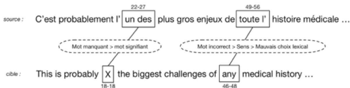
Figure 4. Annotation Representation Example.
