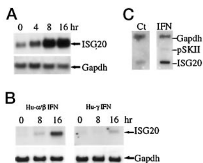
FIG. 1. Northern analysis of IFN-induced ISG20 mRNA. Total RNAs (20 \mu g/lane) were separated on 1.2% formaldehyde-agarose gel, transferred to nylon membrane, and hybridized to a ^{32} P-labeled ISG20 cDNA probe. The same blot was reprobed with a GAPDH probe to ensure that equal amounts of RNA were loaded in each lane. A , time course of ISG20 mRNA induction with HuIFN- \alpha/\beta . Daudi cells were treated with HuIFN- \alpha/\beta (500 units/ml) for the indicated times. B , specificity of ISG20 mRNA induction by HuIFN- \alpha/\beta and HuIFN- \gamma . HeLa cells were treated with HuIFN- \alpha/\beta (500 units/ml) or HuIFN- \gamma (500 units/ml) for the indicated times. C , run-on analysis of transcription elongation of the ISG20 gene. Run-on assays were carried out with nuclei from Daudi cells treated (IFN) or not (control (Ct)) with HuIFN- \alpha/\beta for 16 h. The labeled RNAs were hybridized with a filter containing the indicated probes. pSKII, pBluescript II KS vector.
