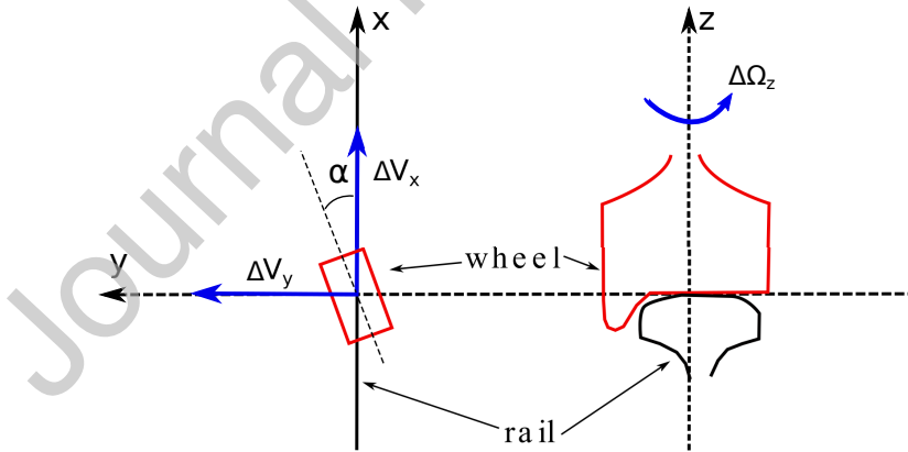
Figure 2: Coordinate system, kinetic variables ( \alpha : angle of attack of the curve, \Delta V_y : imposed lateral sliding velocity, \Delta V_x : imposed longitudinal sliding velocity and \Delta \Omega_z : imposed spin velocity)
