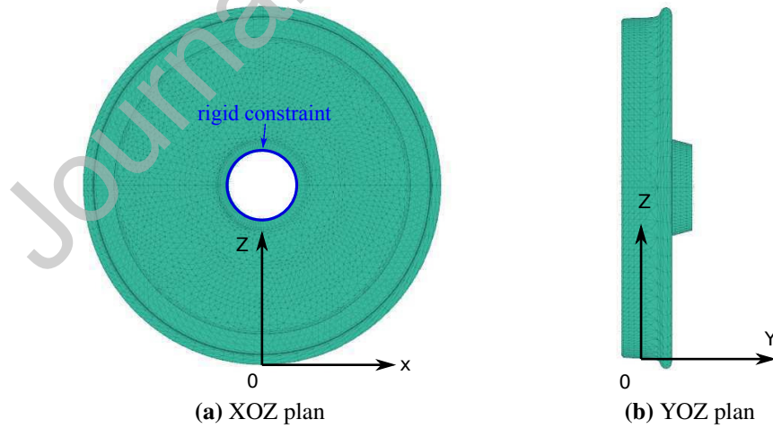
Figure 3: Wheel FEM mesh (wheel of type "Vyksa BA005" with a nominal rolling diameter of 920 mm and a mass of 314 kg) with a rigid constraint applied at the inner face of the hub, where the wheel is connected to the axle.
