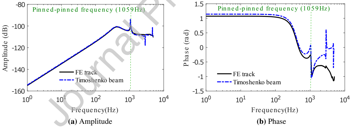
Figure 7: Vertical mobility at contact point (Reference amplitude: 1 m/s/N)
