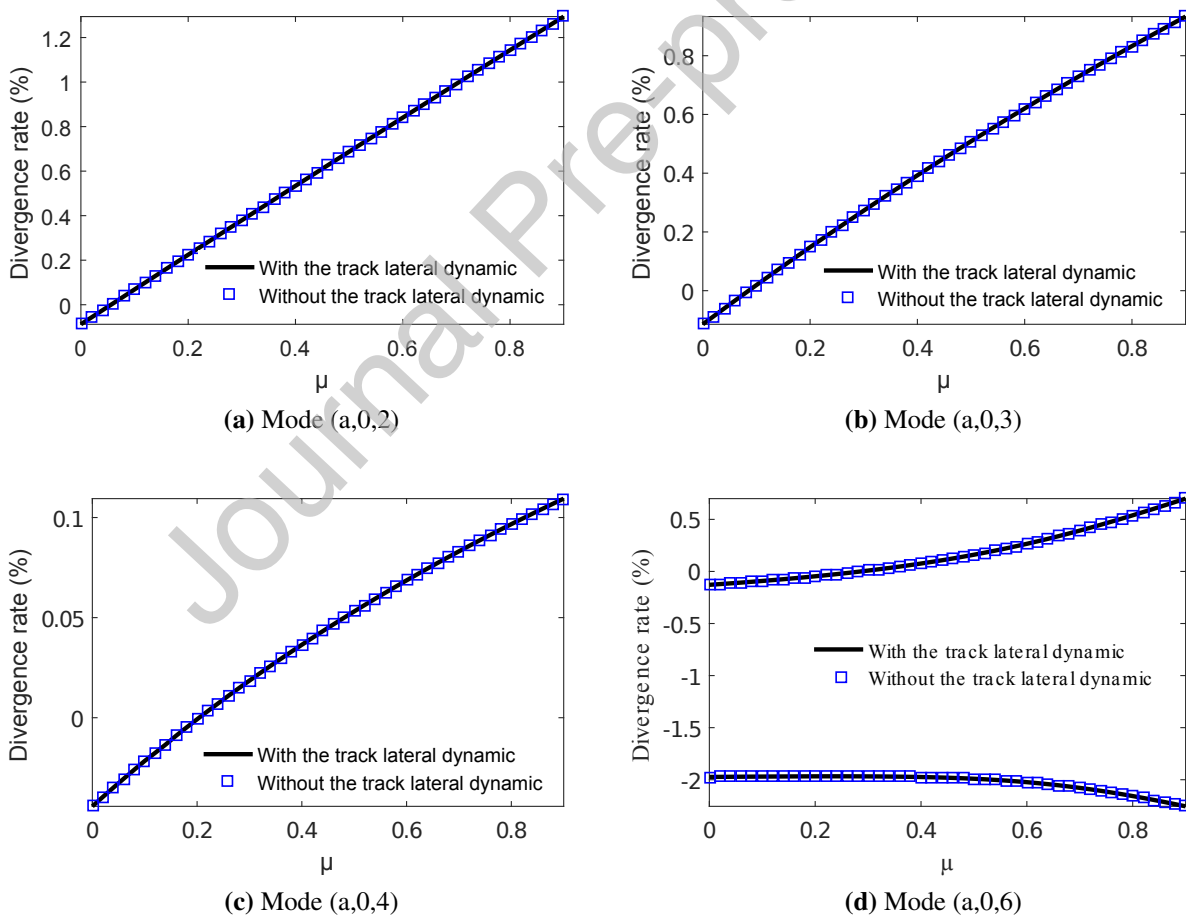
Figure 16: Bifurcation curves of unstable complex modes with and without the lateral flexibility of the rail
