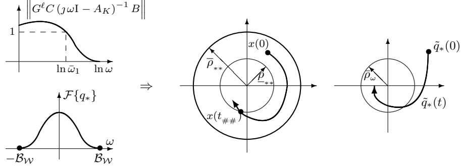
Figure 3: Lemma 3: If \mathcal{F}\{q_*\} = 0 for all |\omega| > \mathcal{B}_{\mathcal{W}} , then: \|\tilde{q}_*(t)\|_\infty \leq k_1 e^{-(\bar{\omega}_1/2)t} \|\tilde{k}_0\| + \rho_\omega , where: \rho_\omega = (\mathcal{B}_{\mathcal{W}}/\bar{\omega}_1)k_4\|q_*(t)\|_\infty ; \bar{\omega}_1 is the bandwidth of (3.2) and \mathcal{B}_{\mathcal{W}} is the bandwidth of q_* (see also (3.24)). Corollary 1: If \bar{\omega}_1 > \mathcal{B}_{\mathcal{W}}\rho_{\#\#} , then any x(t) \in \mathcal{B}_{\bar{\rho}_{**}} is attracted towards the neighborhood \mathcal{B}_{\bar{\rho}_{**}} for t > t_{\#\#} . If \bar{\omega}_1 > \mathcal{B}_{\mathcal{W}}k_4\gamma_2 , then: \|\tilde{q}_*(t)\|_\infty \leq \bar{k}_1 e^{-\alpha_0 t} \|\tilde{k}_0\| + \bar{\rho}_\omega , where: \bar{k}_1 = k_1(\bar{\omega}_1/\mathcal{B}_{\mathcal{W}})/(\bar{\omega}_1/\mathcal{B}_{\mathcal{W}} - k_4\gamma_2) and \bar{\rho}_\omega = (k_4\mu_0\gamma_1/(\bar{\omega}_1/\mathcal{B}_{\mathcal{W}} - k_4\gamma_2))L_X \|\zeta(t)\|_\infty .
