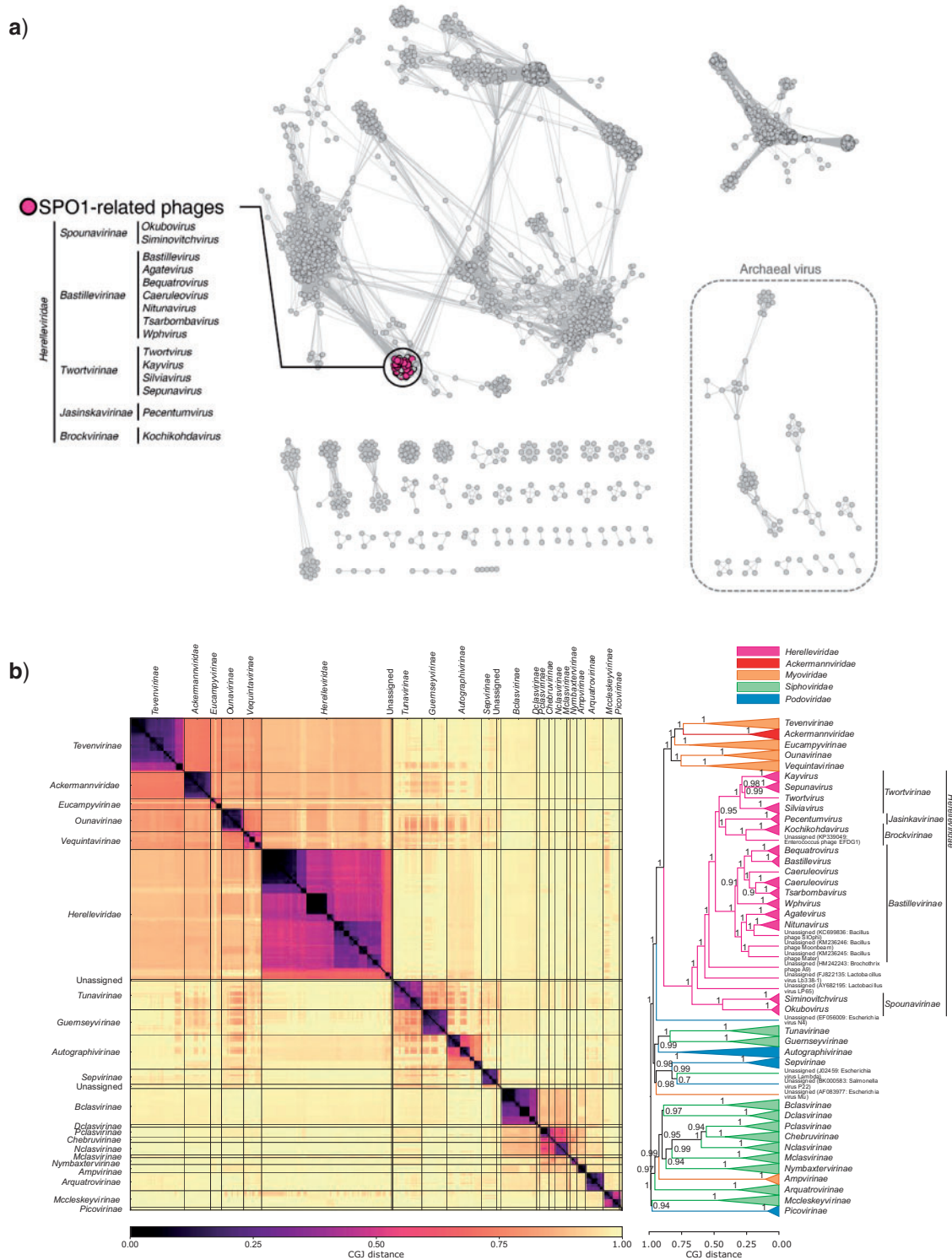
FIGURE 1. a) Network representation of predicted protein content similarity of dsDNA viruses generated with vConTACT v2.0. Viruses are represented as circles (nodes) connected with each other (edges) based on a significant number of shared protein clusters, with more similar genomes displayed closer together on the network. The genomes belonging to the new family Herelleviridae are indicated with a circle. Genomes previously assigned to the subfamily Spounavirinae are indicated in pink. b) Clustering of dsDNA bacteriophages that possess subfamily assignments in the order Caudovirales generated with GRAViTy, darker colors in the heatmap represent higher degrees of similarity between genomes. The phages are clustered using UPGMA into a dendrogram, showing bootstrap values (100 pseudoreplicates) on each branch.
