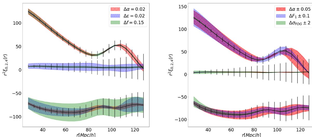
Figure 8. Left-hand panel: Model variations for \Delta f , \Delta\alpha , and \Delta\epsilon compared to the error bars coming from covariance: the behaviour for the monopole (top), the hexadecapole (middle), and the quadrupole (bottom). The variations in \epsilon have a large impact on the hexadecapole, while the variations in \alpha and growth factor are of the same order of magnitude for the hexadecapole. This behaviour explains why fits are driven by \epsilon when the hexadecapole is taken into account. Right-hand panel: Model variations for \Delta F , \Delta\alpha , and \Delta\sigma_{\text{FOG}} compared to the errors produced by covariance: the behaviour for the monopole (top), the hexadecapole (middle), and the quadrupole (bottom).
