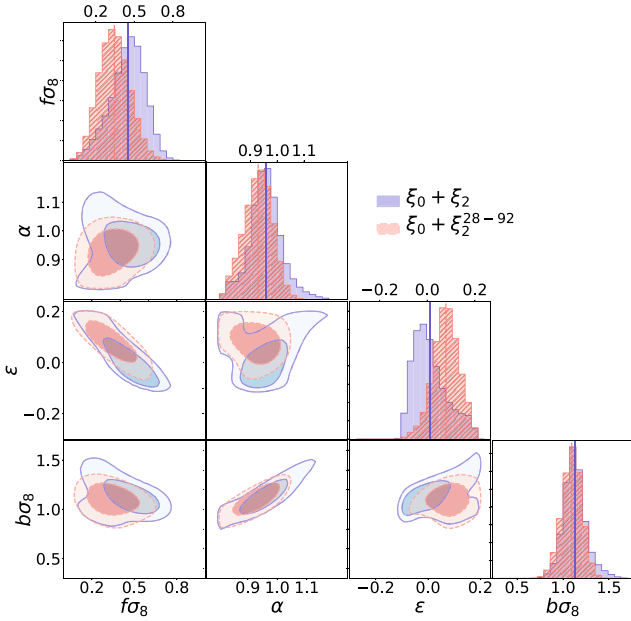
Figure 17. The shaded regions show the 1-2\sigma confidence surfaces found by our MCMC chains for the RSD-AP parameters for the \xi_0 + \xi_2 space in the fiducial range (blue solid) and when excluding the large scales in quadrupole (red dashed). The confidence contours for the growth factor f\sigma_8 , the linear bias b\sigma_8 , the dilatation parameter \alpha , and the warping parameter \epsilon are indicated, along with their 1D distributions. The dashed lines of each histogram are the mean values found by the MCMC chain.
