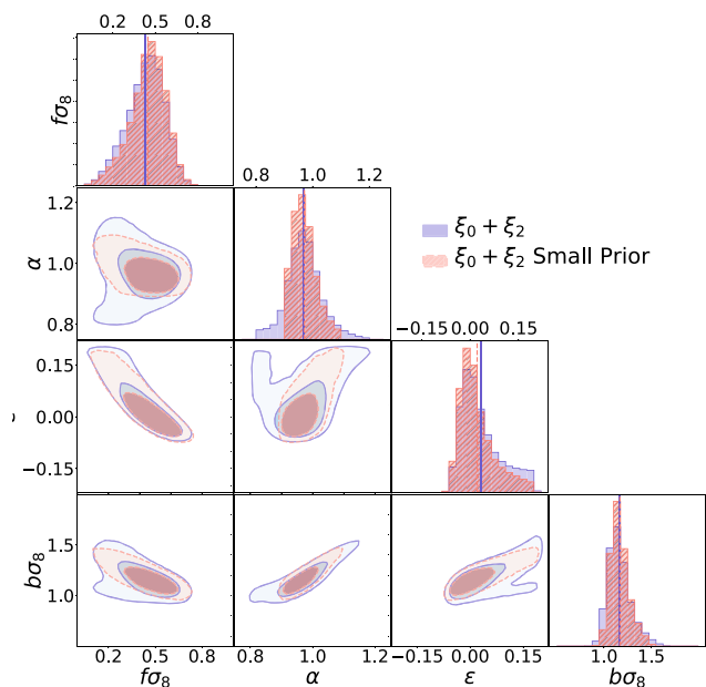
Figure A3. This plot is equivalent to Fig. 17, here we are presenting the MCMC chains of two fits to the RSD-AP parameters in the \xi_0 + \xi_2 space done with different priors in \alpha . The solid-line contours use the priors quoted in Table 8 for all parameters but F_2 that is set to zero. The red dashed-line contours have smaller priors on \alpha which are reduced to [0.9, 1.1] and also set F_2 to zero.
