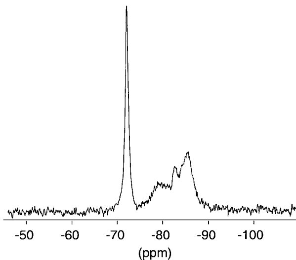
Figure 10 ^1\text{H}\text{-}^{29}\text{Si} cross polarization (10 ms contact time) NMR spectrum of \text{C}_3\text{S} hydrated with quartz at 120^\circ\text{C} during 4 days under 1000 bar.
