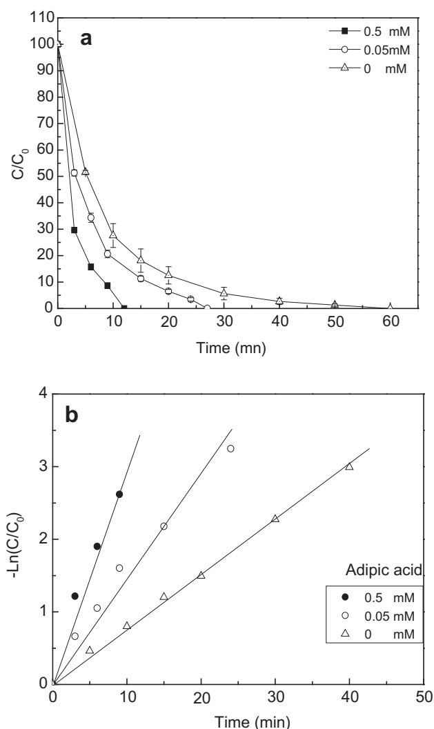
Fig. 7 Photocatalytic reduction of 10^{-4} M K_2Cr_2O_7 aqueous solution using 3 mg of CuS NSs in the presence of adipic acid 0 mM (pH = 6.9), 0.05 mM (pH = 6.3) and 0.5 mM (pH = 4.5) under visible light irradiation (a) and the corresponding degradation kinetics with first order linearity of -\ln(C/C_0) = kt (b).
