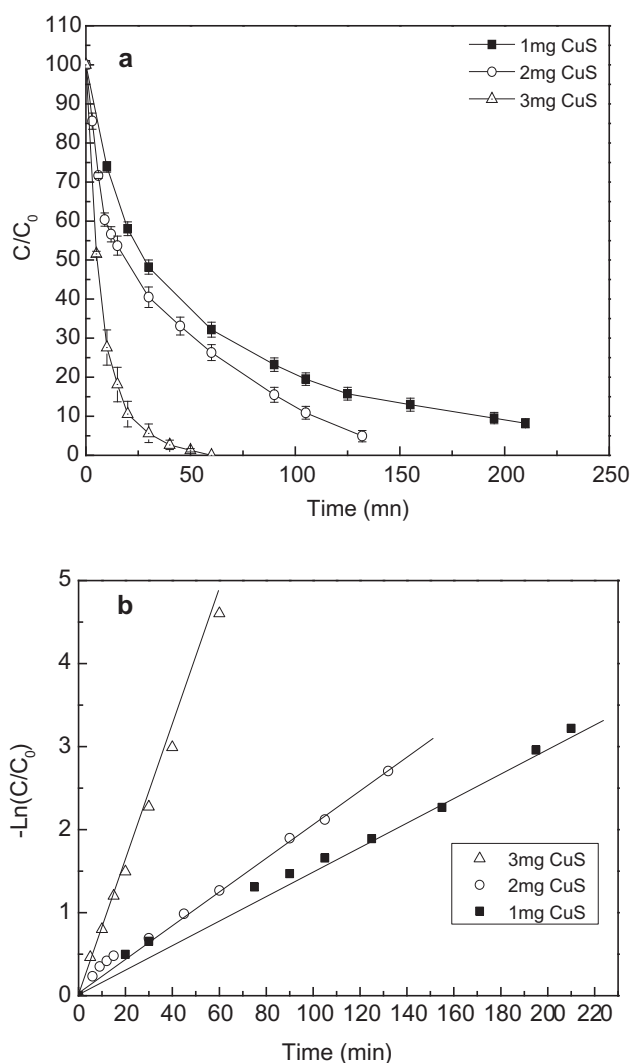
Fig. 6 Photocatalytic reduction of 10^{-4} M K 2 Cr 2 O 7 aqueous solution in the presence of CuS NSs (1, 2 and 3 mg) under visible light irradiation (a) and the corresponding degradation kinetics with first order linearity of -\ln(C/C_0) = kt (b).
