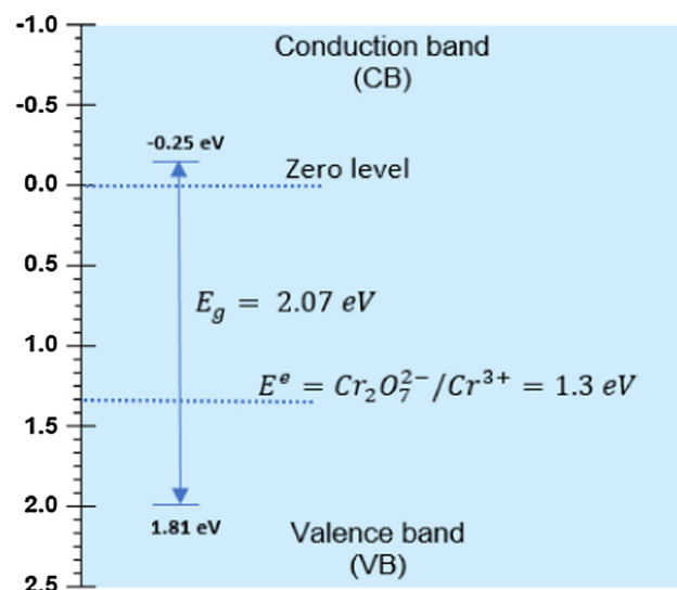
Scheme 1 Diagram of the energy band structure of CuS NSs.
