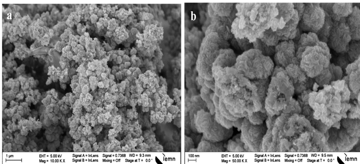
Fig. 2 Scanning electron microscopy (SEM) images of as-prepared CuS NSs.
