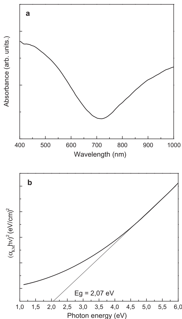
Fig. 4 (a) Optical absorption spectrum of CuS NSs (1 mg in 4 mL H 2 O) and (b) plot of the square of absorbance (\alpha_{KM} hv)^2 versus photon energy h\nu .
