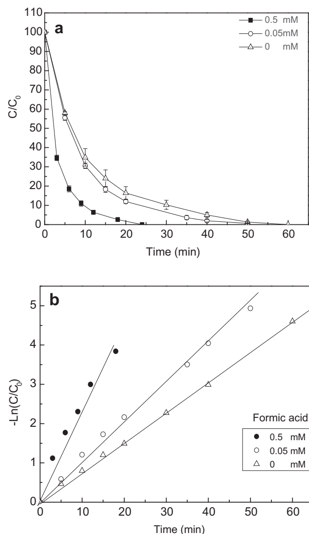
Fig. 8 Photocatalytic reduction of 10^{-4} M K_2Cr_2O_7 aqueous solution using 3 mg of CuS NSs in the presence of formic acid 0 mM (pH = 6.9), 0.05 mM (pH = 6.16) and 0.5 mM (pH = 4.12) under visible light irradiation (a) and the corresponding degradation kinetics with first order linearity of -\ln(C/C_0) = kt (b).
