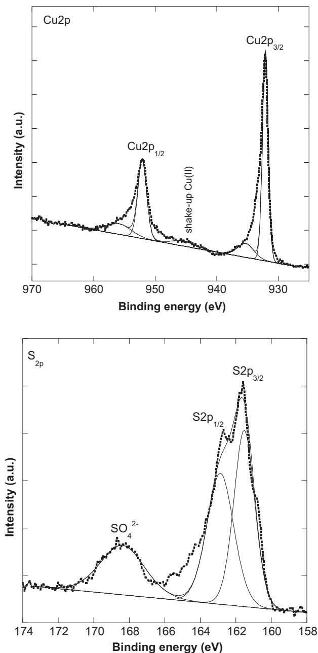
Fig. 5 (a) Cu 2p and (b) S 2p high resolution X-ray photoelectron spectroscopy (XPS) of CuS NSs.
