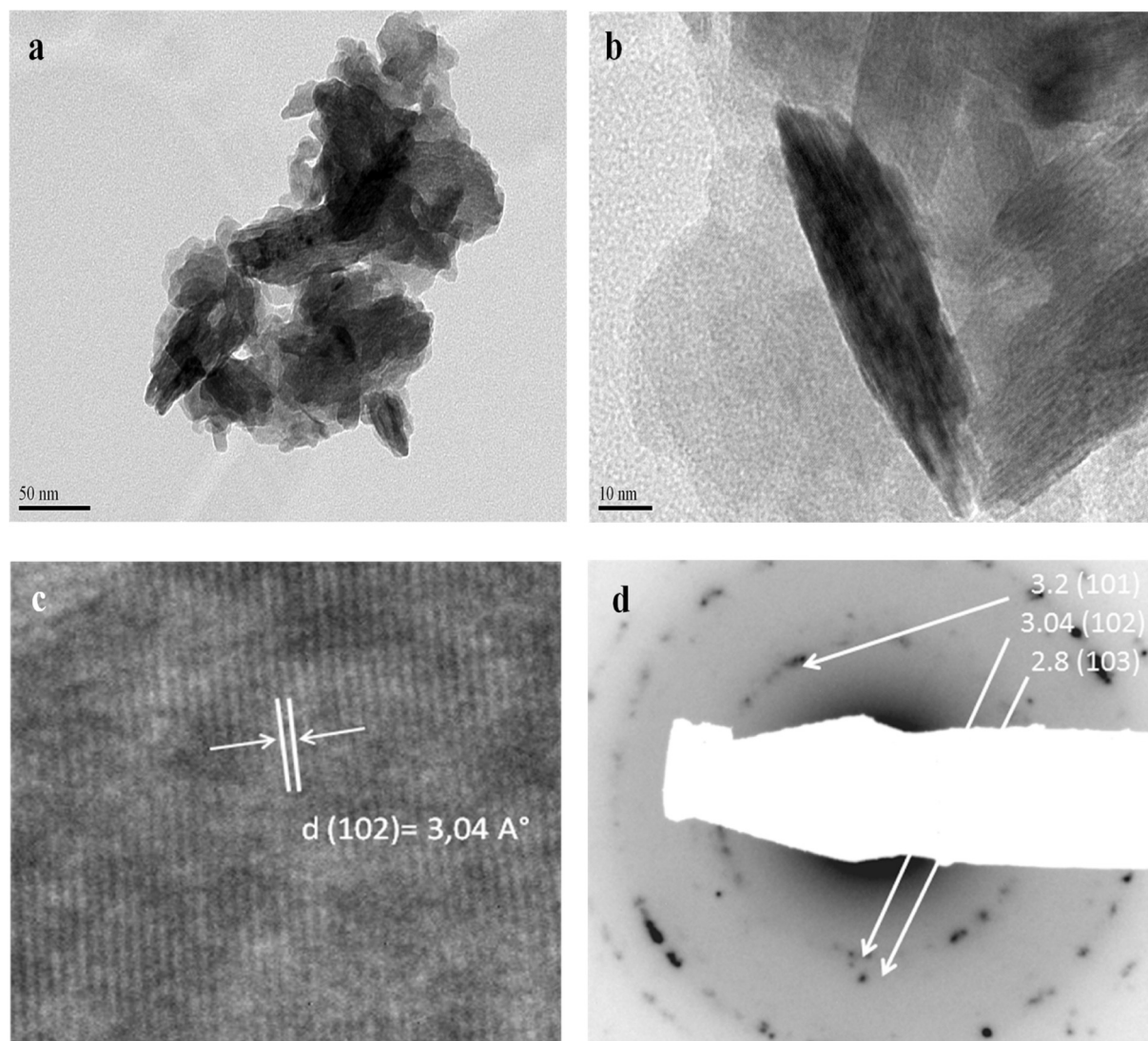
Fig. 3 (a and b) Typical TEM images, (c) HRTEM image showing lattice planes, and (d) selected area electron diffraction (SAED) pattern of CuS NSs, dotted pattern confirmed the crystalline nature of CuS NSs.
