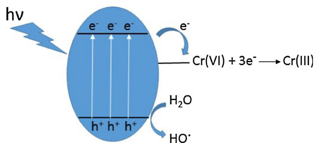
Scheme 2 Plausible mechanism of Cr(VI) reduction using CuS NSs photocatalyst under visible light irradiation.
