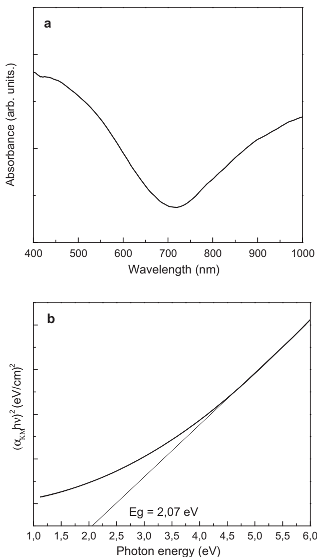
Fig. 4 (a) Optical absorption spectrum of CuS NSs (1 mg in 4 mL H 2 O) and (b) plot of the square of absorbance (\alpha_{KM} h\nu)^2 versus photon energy h\nu .
