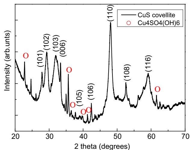
Fig. 1 X-ray diffraction pattern of as-prepared CuS NSs.
