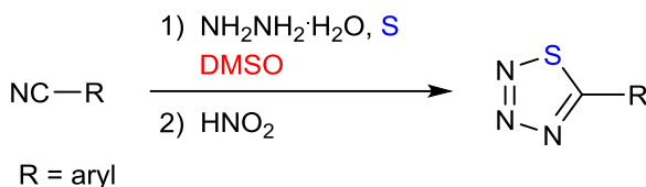
Scheme 1. Overview of synthetic approaches to 1,2,3,4-thiazoles.
