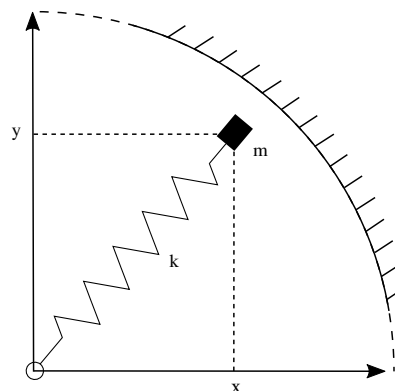
FIGURE 3 – Ressort tournant
