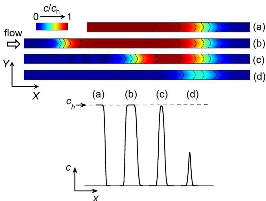
FIGURE 2 | Top: Side view of simulated concentration profiles at a given time between the two working electrodes E1 and E2 in a linear microchannel: front (a), plug (b), and peak (c,d). The black solid curves on the concentration profiles represent isoconcentration lines. Bottom: Concentration variations along X-axis illustrating the different types of concentration gradient. c_h is the maximal concentration reached within a front (a) or plug (b).
