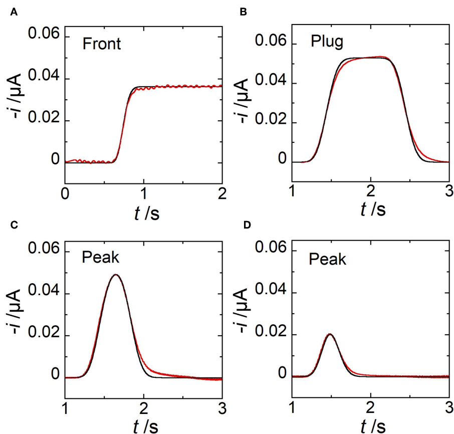
FIGURE 7 | Comparison between simulated (black lines) and experimental (red lines) current responses monitored at electrode E2. (A) Case of a concentration front. (B) Case of a concentration plug with t_{\text{pulse}} = 1 s. Estimated w_g = 1860 \mu\text{m} . (C) Case of a concentration peak with t_{\text{pulse}} = 0.4 s. Estimated w_g = 744 \mu\text{m} . (D) Case of a concentration peak with t_{\text{pulse}} = 0.1 s. Estimated w_g = 446 \mu\text{m} . In (A) w_{E1} = 97 \mu\text{m} , w_{E2} = 17 \mu\text{m} , g = 1000 \mu\text{m} , h = 20 \mu\text{m} , l = 510 \mu\text{m} , u_{\text{av}} = 0.86 \mu\text{L min}^{-1} , and c_0 = 0.63 \text{ mM} . In (B–D) w_{E1} = 200 \mu\text{m} , w_{E2} = 30 \mu\text{m} , g = 2600 \mu\text{m} , h = 24 \mu\text{m} , l = 790 \mu\text{m} , u_{\text{av}} = 2.12 \mu\text{L min}^{-1} , and c_0 = 0.38 \text{ mM} . In (A–D) , each curve is related to a single experiment.
