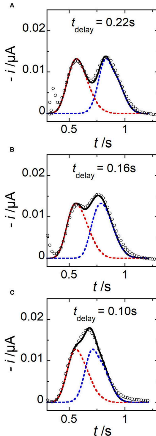
FIGURE 9 | Comparison between simulated (lines) and experimental (symbols) current responses monitored at electrode E2 in the case of two consecutive peaks generated for three different t_{\text{delay}} . (A) t_{\text{delay}} = 0.22 \text{ s} . (B) t_{\text{delay}} = 0.16 \text{ s} . (C) t_{\text{delay}} = 0.10 \text{ s} . In (A–C) , t_{\text{pulse}} = 0.06 \text{ s} , w_{E1} = 200 \mu\text{m} , w_{E2} = 30 \mu\text{m} , g = 400 \mu\text{m} , h = 20 \mu\text{m} , l = 790 \mu\text{m} , c_0 = 0.33 \text{ mM} , and u_{\text{av}} = 1 \mu\text{L min}^{-1} . Each simulated peak is plotted in dashed line (red or blue). The solid line corresponds to the sum of peak contributions. Each current response is related to a single experiment.
