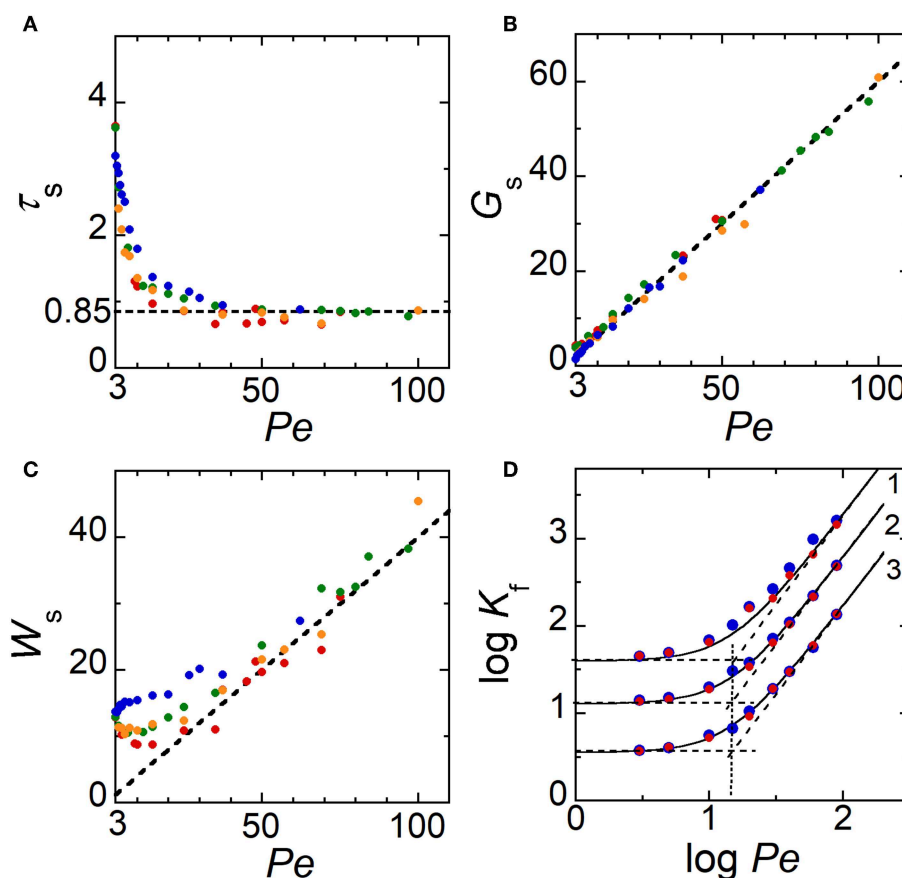
FIGURE 4 | (A–C) Theoretical variations of \tau_s , G_s , and W_s as a function of Pe for several electrode sizes W_{E1} . The dashed lines correspond to \tau_s = 0.85 , G_s = 0.6 Pe , and W_s = 0.4 Pe , respectively. (D) Variation of \log K_f as a function of \log Pe for three couples of isoconcentration lines: 1 ( C_{99} , C_{01} ); 2 ( C_{90} , C_{10} ), and 3 ( C_{75} , C_{25} ). The solid lines correspond to Equation (5) when \gamma_f = 40 ( C_{99} , C_{01} ), \gamma_f = 13 ( C_{90} , C_{10} ), and \gamma_f = 3.6 ( C_{75} , C_{25} ). Dashed lines represent the two limiting cases. In (A–C) , symbols correspond to data evaluated from numerical simulations with W_{E1} = 9.85 (blue), 4.85 (orange), 2.85 (green), and 0.85 (red). In (D) , W_{E1} = 10 (blue) and 1 (red).
