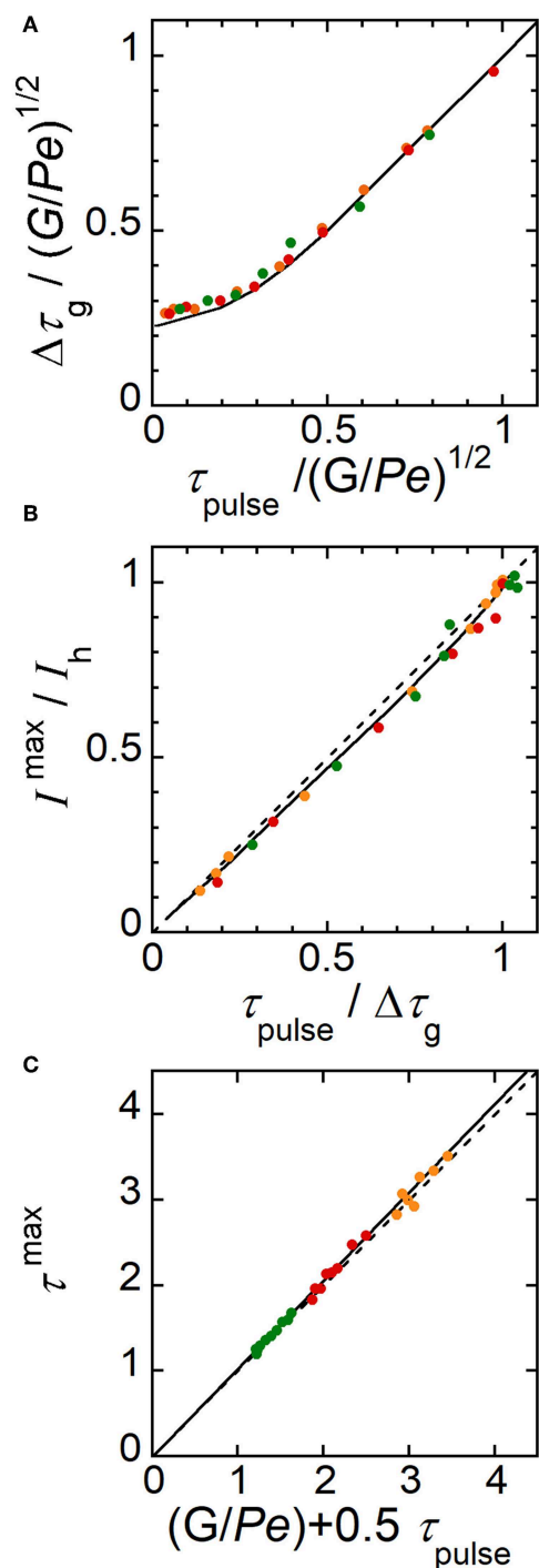
FIGURE 8 | Characteristic parameters evaluated theoretically (solid lines) and experimentally (symbols) from current responses monitored at electrode E2. (A) Plot of \Delta\tau_g / (G/Pe)^{1/2} as a function of \tau_{\text{pulse}} / (G/Pe)^{1/2} . (B) Plot of I^{\text{max}} / I_h as a function of \tau_{\text{pulse}} / \Delta\tau_g . The dashed line is the equation I^{\text{max}} / I_h = \tau_{\text{pulse}} / \Delta\tau_g . (C) Plot of \tau^{\text{max}} as a function of (G/Pe) + 0.5\tau_{\text{pulse}} . The dashed line is the equation \tau^{\text{max}} = G/Pe + 0.5\tau_{\text{pulse}} . In (A–C) , experimental flow rate u_{\text{av}} = 1.40 \mu\text{L min}^{-1} (green), 2.12 \mu\text{L min}^{-1} (red), and 3.27 \mu\text{L min}^{-1} (orange). w_{E1} = 200 \mu\text{m} , w_{E2} = 30 \mu\text{m} , g = 2600 \mu\text{m} , h = 24 \mu\text{m} , l = 790 \mu\text{m} , and c_0 = 0.38 \text{ mM} . t_{\text{pulse}} ranged from 0.1 to 1 s. In (A–C) , each data is related to a single experiment.
