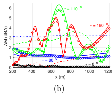
with respect to x at z = 2 m in a neutral atmosphere at \tau = 0^\circ (downwind), \tau = 80^\circ , \tau = 110^\circ , and \tau = 180^\circ (upwind): Amiet-PE (-), point source approximation (--), MM with 19 heights (o). Color online.
