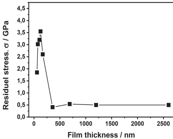
Figure 6. Residual stress of Cr films before annealing.
