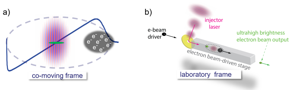
Figure 10. (a) Collinear Trojan Horse schematic in the co-moving frame; and (b) laboratory frame. The laser focusing pulse releases ultracold electrons (green) from the high ionization threshold medium, which then briefly fall back and are trapped in the back part of the accelerating blowout.
