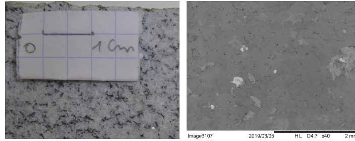
Figure 1 Picture and microscopic view by Scanning Electron Microscopy (x40) of the used granite in this study.
