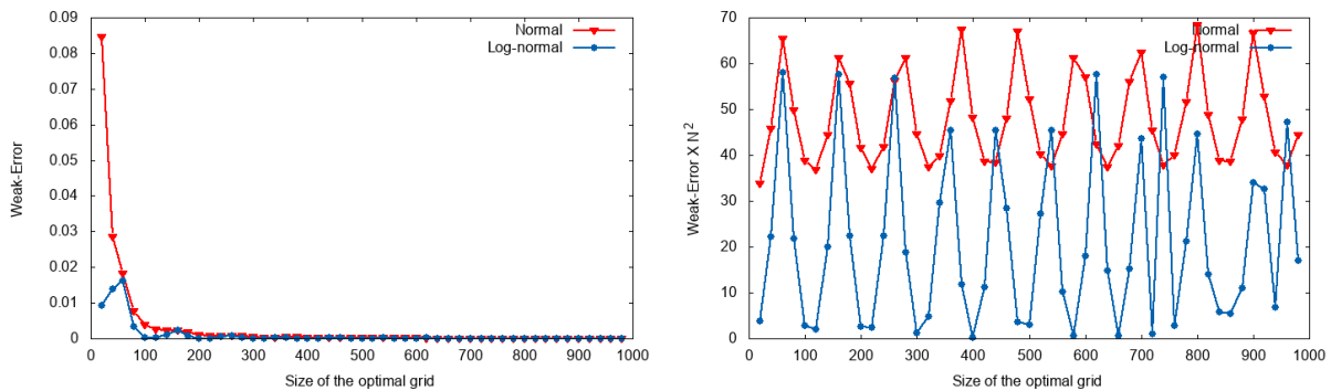
(a) N \mapsto |I_0 - \mathbb{E}[f(\hat{Z}^N)]| ( \blacktriangledown ) and N \mapsto |I_0 - \mathbb{E}[\varphi(\hat{X}^N)]| ( \bullet ) (b) N \mapsto N^2 \times |I_0 - \mathbb{E}[f(\hat{Z}^N)]| ( \blacktriangledown ) and N \mapsto N^2 \times |I_0 - \mathbb{E}[\varphi(\hat{X}^N)]| ( \bullet )
