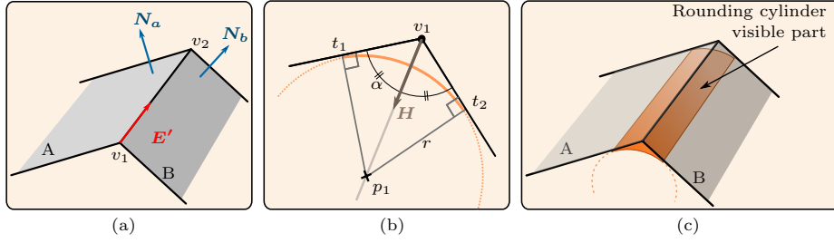
Fig. 3: A rounding cylinder for an edge (v_1, v_2) is associated with adjacent faces A and B . (a) A and B have respective normals N_a and N_b , H = -(N_a + N_b)/|N_a + N_b| . (b) p_1 (resp. p_2 ) is defined from vertex v_1 (resp. v_2 ) and H ; (c) The visible area of the rounding cylinder defined by the axis (p_1, p_2) and the cylinder radius r is defined by the user.
