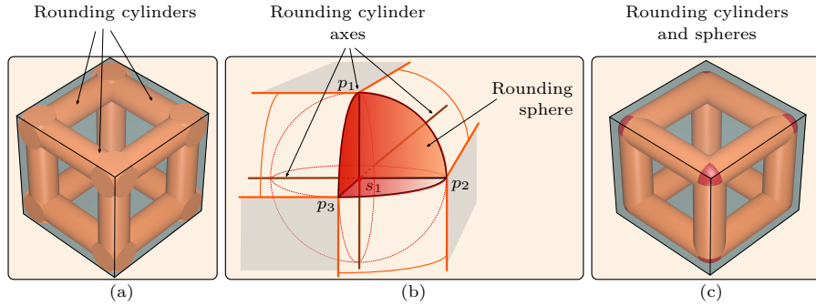
Fig. 4: (a) Set of rounding cylinders for a cube. (b) Axes of cylinders cross at a point, defining a rounding sphere center ( s_1 is the sphere center associated with p_1 , p_2 , and p_3 ). (c) Final configuration with rounding spheres and rounding cylinders.
