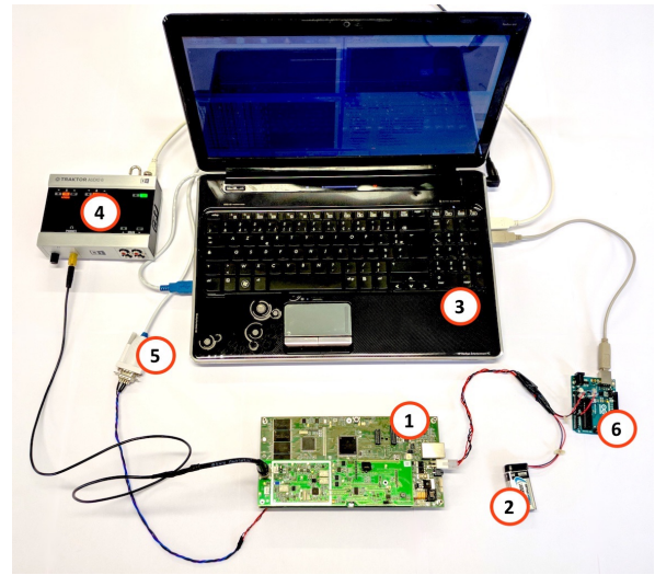
Fig. 3. Experimental setup.
