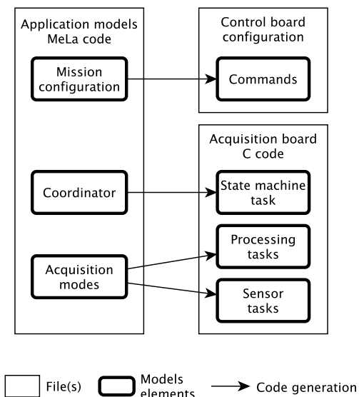
Fig. 2. Code generation from MeLa applications.
