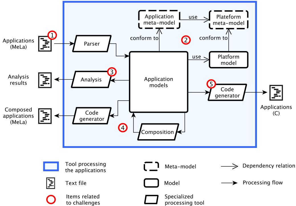
Fig. 1. Modeling of applications.
