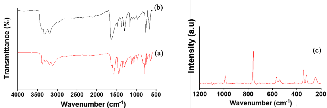
Figure 2. Infrared spectra of the organic part DAP (a) and the hybrid [\text{C}_5\text{H}_8\text{N}_3]_2\text{SbCl}_5 (b). Raman spectrum of [\text{C}_5\text{H}_8\text{N}_3]_2\text{SbCl}_5 (c).
