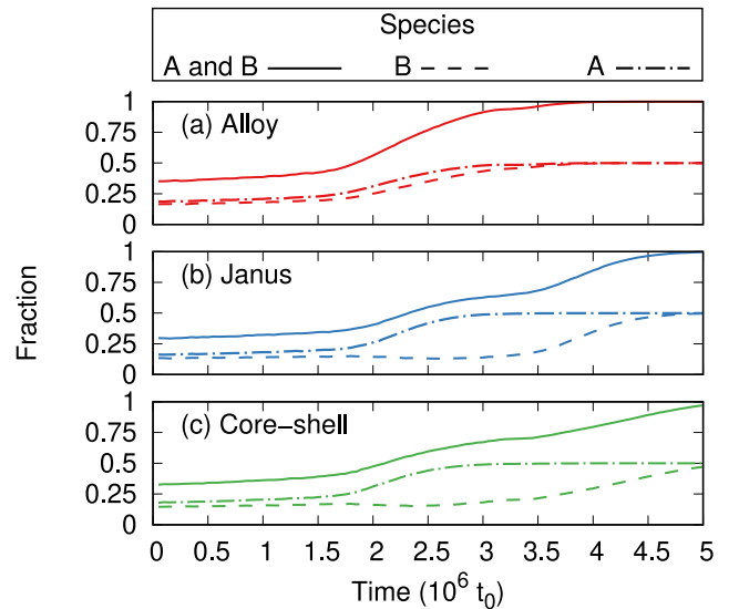
FIG. 6. Species-resolved fraction of atoms within NPs obtained at a quench duration of 5 \times 10^6 t_0 in the (a) alloy, (b) Janus and (c) core-shell cases.
