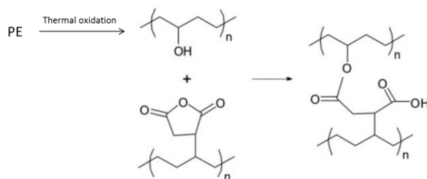
Scheme 4. Reaction between hydroxyl groups of thermo-oxidized PE units and maleic anhydride group of MA-g-PE.
