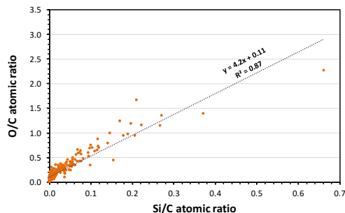
Figure 3: EMPA data for 10 UCAMMs showing the correlation of O/C vs. Si/C. The O/Si obtained by regression is \sim 4 .
