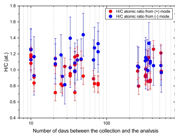
Fig. 5. H/C atomic ratio of the 35 considered analyses for the two registration modes (red and blue points are positive and negative analyses, respectively) as a function of the time between the collection date of the cometary particles and their analysis.
