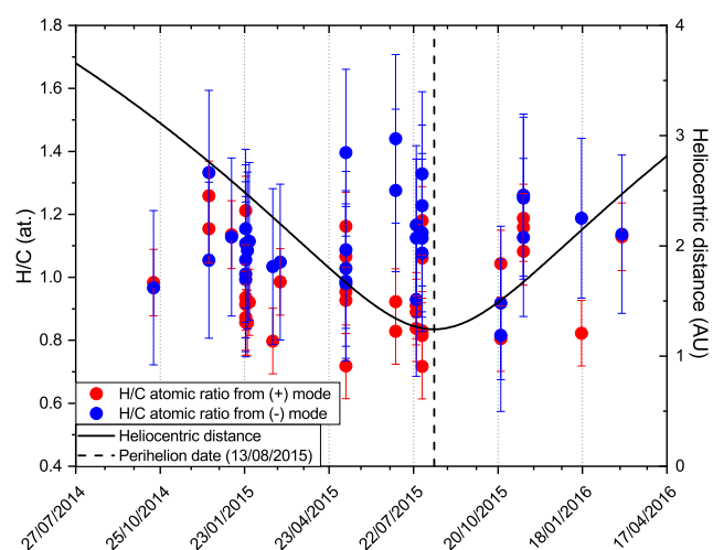
Fig. 4. H/C atomic ratio of the 35 considered analyses as a function of the collection date of the cometary particles for the two registration modes (red and blue points are positive and negative analyses, respectively). The black curve and the dashed line represent the heliocentric distance of 67P and the date at the perihelion (13 August 2015), respectively.
