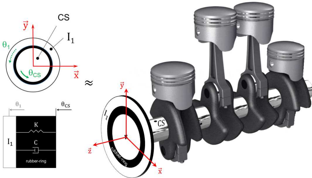
Figure 2. Torsional vibration damper and its schematic diagrams.
