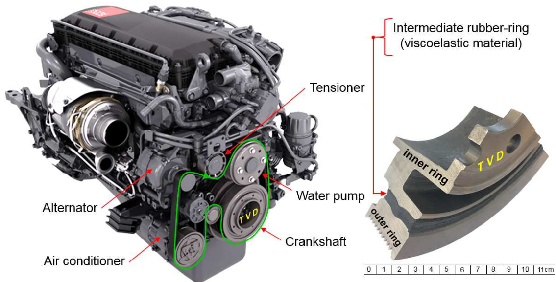
Figure 1. Serpentine poly-v belt of a FEAD with its TVD pulley.
