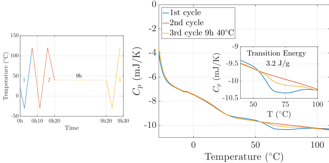
Figure 5: Thermal characterization of PVB with three successive temperature ramps - a: thermal history; b: heat capacity
