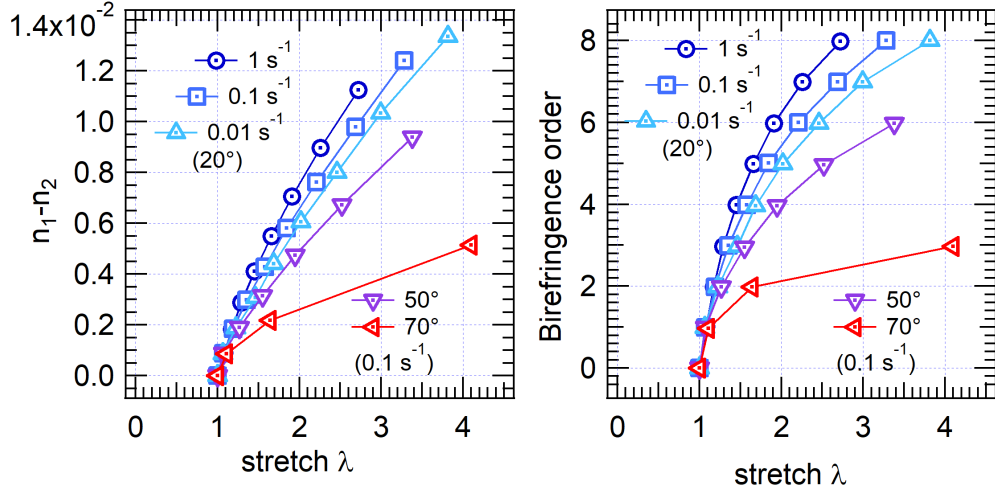
Figure 10: Birefringence ( n_1 - n_2 ) (left) and fringe order N (right) as a function of stretch \lambda . The birefringence was calculated from the relation (n_1 - n_2)h_0 = N l_{opt}\sqrt{\lambda} to account for sample thinning at constant volume. It is strongly dependent upon temperature and moderately dependent upon stretch rate, but not proportional to stress.
