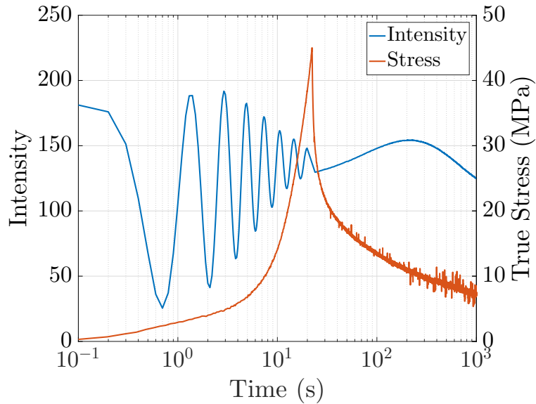
Figure 11: After loading at 20°C and 0.01 s -1 stretch rate, the strain is kept constant at the maximal value of 200% ( \lambda = 3 ). Stress is found to relax rapidly while birefringence order changes only by about half a unit.
