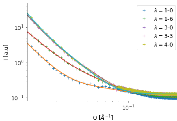
Figure 7: SAXS-WAXS spectra of PVB stretched at \lambda = 1, 1.6, 3, 3.3, 4 at 23^\circ\text{C} in the direction of the elongation. The solid lines correspond to the best fits defined by equation 2.
