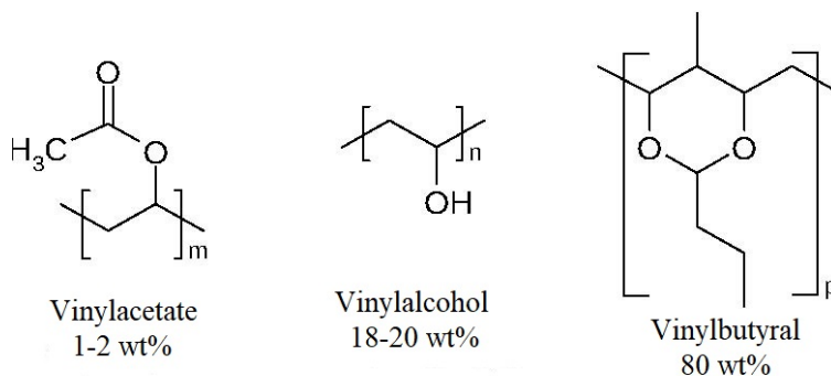
Figure 1: PVB monomers.
