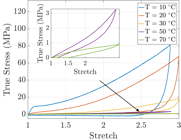
Figure 4: Temperature dependence of PVB large strain response in uniaxial tension cycles performed at 0.1 \text{ s}^{-1} up to 200% deformation ( \lambda = 3 ). The inset is a zoom for T = 50 and 70^\circ\text{C} .
