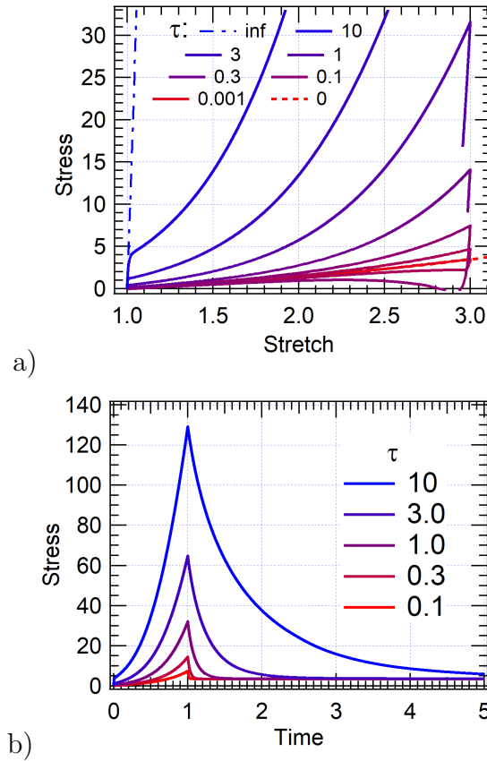
Figure 15: Creep based numerical model with strain hardening: a) stress-stretch relation with various creep times and constant loading time. The limit cases are elastic with the short time ( \tau = \infty ) or long time modulus ( \tau = 0 ); b) stress relaxation curves for the same parameters.
