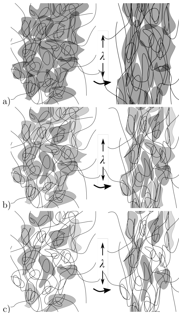
Figure 13: Schematic view of the heterogeneous structure sharing the same PVB macro-molecules, following Schaefer et al. 16 The grey second phase domains present a high density of H-bonds, they are stiffer and with a reduced mobility (the various shades of gray here reflect some variability in the exact structure and dynamics), while the white domains contain fewer H-bonds, more plasticizer and are softer. Upon stretching, the deformation of the domains result in anisotropic response in the SAXS-WAXS signal (Fig. 6). At low temperature (10°C) or high strain rate, the stiffer domains percolate (a). At room temperature and moderate strain rate, close packing implies significant deformation of the stiff domains during stretching (b) and the material retains most of its plastic nature, with high stress levels, strain hardening and birefringence induced by molecular orientation during plastic like flow. At elevated temperature (70°C), packing is looser, and the material responds as a loosely crosslinked viscoelastic matrix (c).
