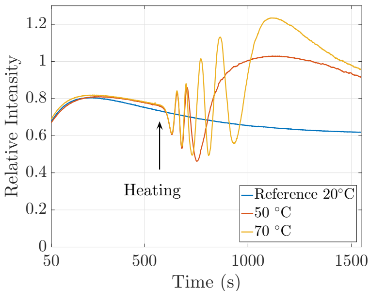
Figure 12: Relaxation with temperature step: birefringence is reduced when temperature is raised from 20°C to 50°C or 70°C during the hold period.
