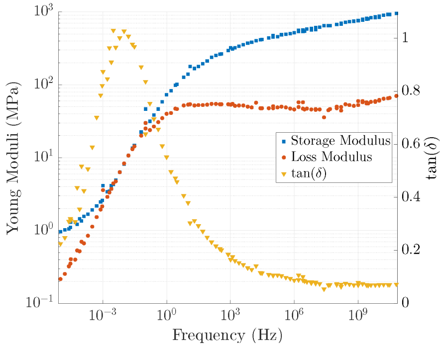
Figure 2: Small strain (0.01%) dynamic response of PVB reconstructed through time temperature superposition with frequency ranging from 0.01 Hz to 1 Hz and temperature from 40 °C to 60 °C – reference temperature 20 °C.
