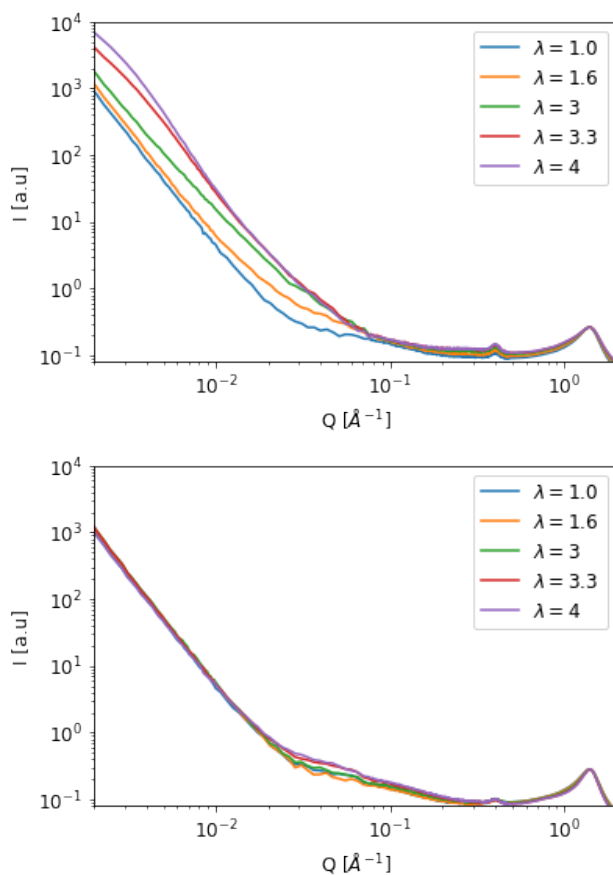
Figure 6: SAXS/WAXS spectra of PVB stretched at \lambda = 1, 1.6, 3, 3.3, 4 at 23^\circ\text{C} in the direction of the elongation (top) and perpendicular to it (bottom).
