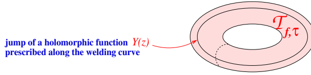
FIG. 5: Inhomogeneous Riemann-Hilbert problem on \mathcal{T}_{f,\tau}
