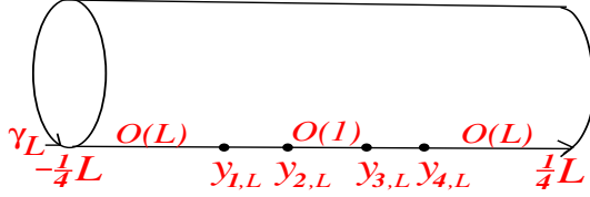
FIG. 3: Euclidian cylinder
