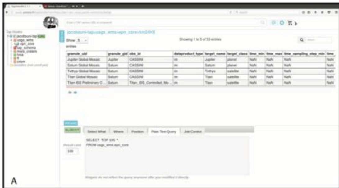
Figure 9: EPN-TAP table of the USGS planetary maps service, as seen in TapHandle.
