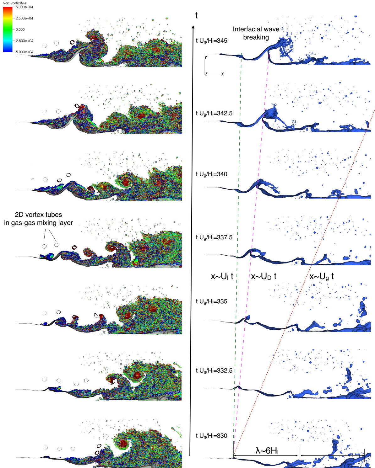
FIGURE 2. Development of the interfacial wave and coherent vortical structures.
