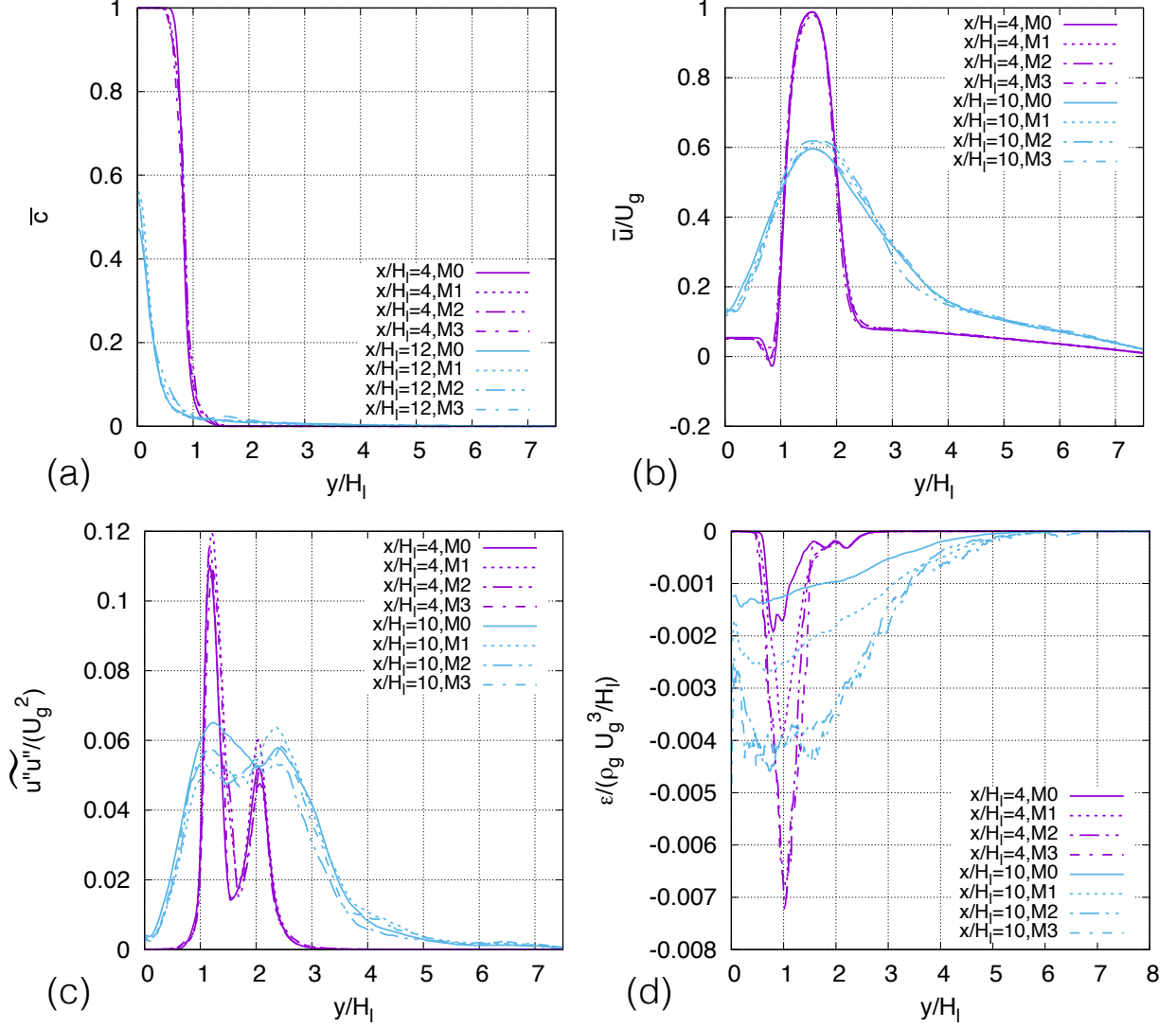
FIGURE 19. Statistical convergence studies for multiphase turbulence statistics.
