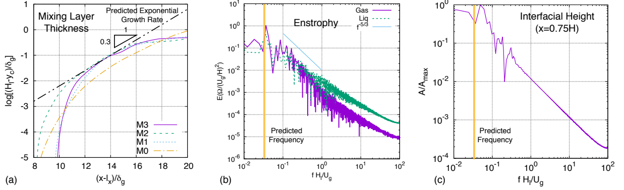
FIGURE 15. (a) Spatial growth of the numerically measured mixing layer thickness, compared with the exponential growth predicted using the maximum spatial growth rate; and the dominant frequency indicated by the numerical results of (b) the spectra of overall liquid and gas enstrophy of the whole domain and (c) the spectra of the interfacial height at x/H_l = 0.75 , compared with the predicted value by stability analysis.
