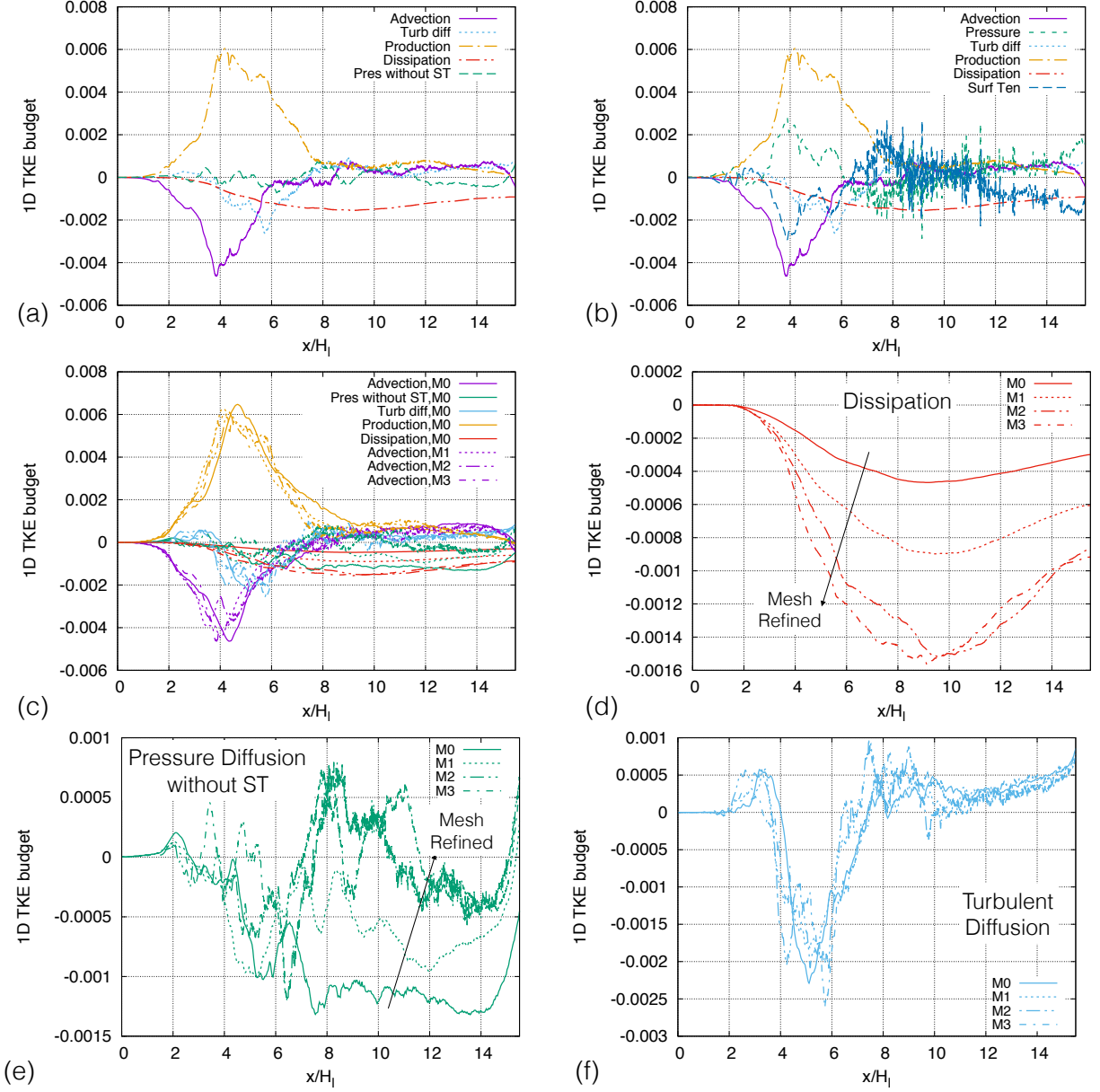
FIGURE 9. One-dimensional turbulence kinetic energy budget along streamwise direction. The terms in Eq. (3.19) are normalized by \rho_g U_g^3 / H_l and averaged over domain height L_y . Figures (a) and (b) are TKE budget with and without the Laplace pressure contribution subtracted from the pressure diffusion term; while figure (c) shows the TKE budget computed with different mesh resolutions.
