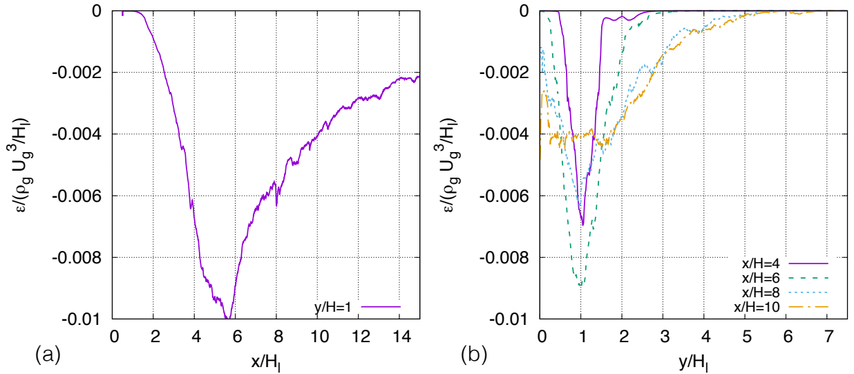
FIGURE 11. Profiles of turbulent kinetic energy dissipation along the lines (a) y/H_l = 1 and (b) x/H_l = 4, 6, 8, and 10 .
