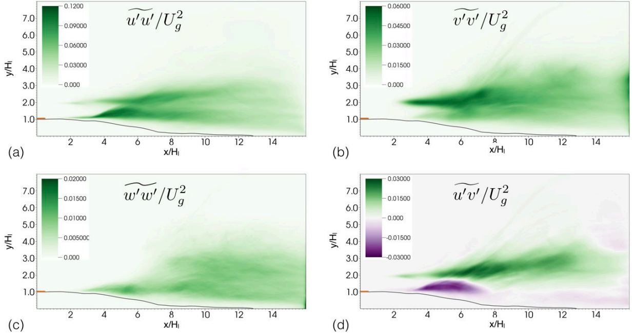
FIGURE 7. Reynolds stresses divided by the average density for Favre averaging. The black curve corresponds to \bar{c} = 0.5 . The orange rectangle near the inlet represents the separator plate.
