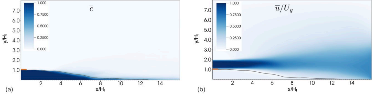
FIGURE 4. Average liquid volume fraction and u -velocity. The black curve corresponds to \bar{c} = 0.5 . The orange rectangle near the inlet represents the separator plate.
