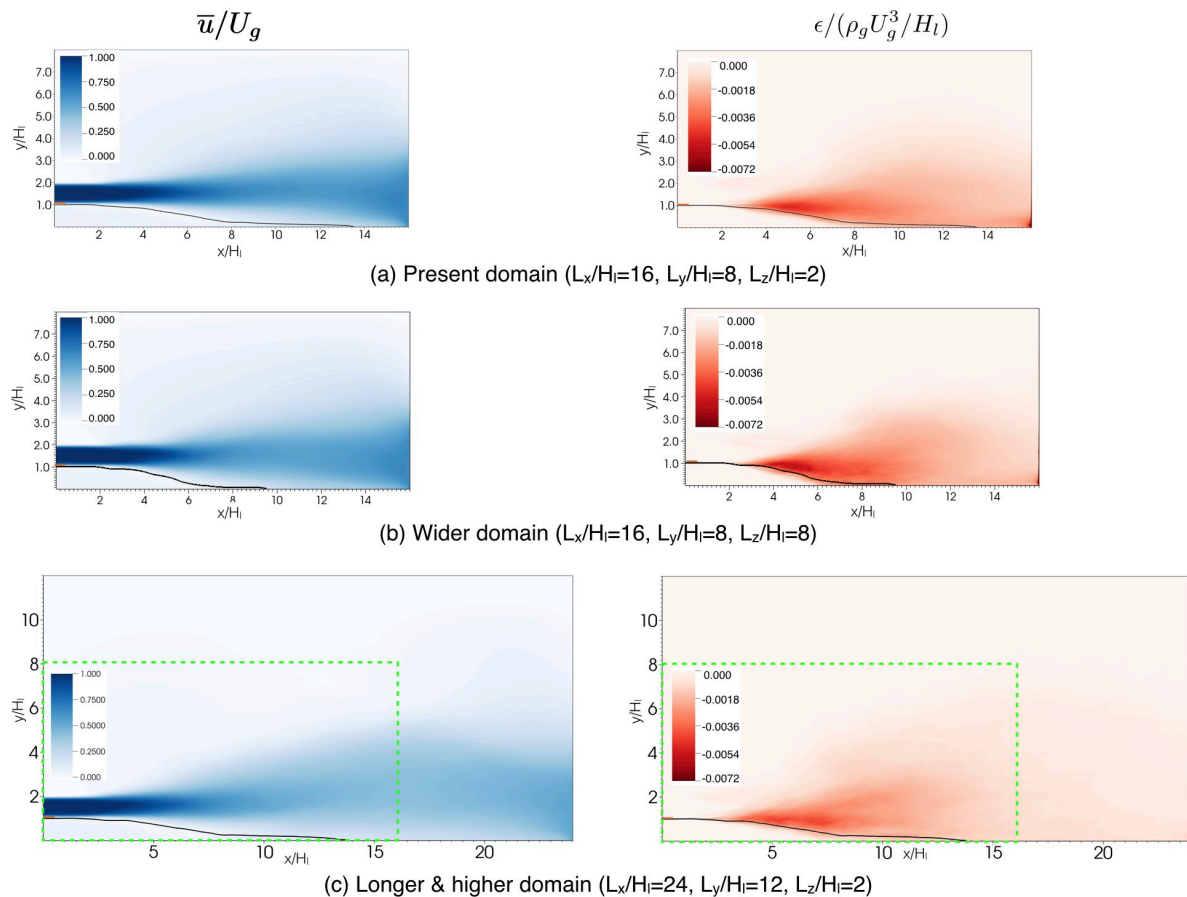
FIGURE 22. Comparison of results for different domain size: (a) the present domain ( L_x/H_l = 16 , L_y/H_l = 8 , L_z/H_l = 2 ), (b) the wider domain ( L_x/H_l = 16 , L_y/H_l = 8 , L_z/H_l = 8 ), and (c) the longer and higher domain ( L_x/H_l = 24 , L_y/H_l = 12 , L_z/H_l = 2 ). The results presented here are for the M1 mesh resolution, i.e. , H_l/\Delta = 64 . The left and right columns are the mean velocity and the turbulent dissipation, respectively. The black curve corresponds to \bar{c} = 0.5 . The box with green dashed lines indicate the present domain size. The orange rectangle near the inlet represents the separator plate.
