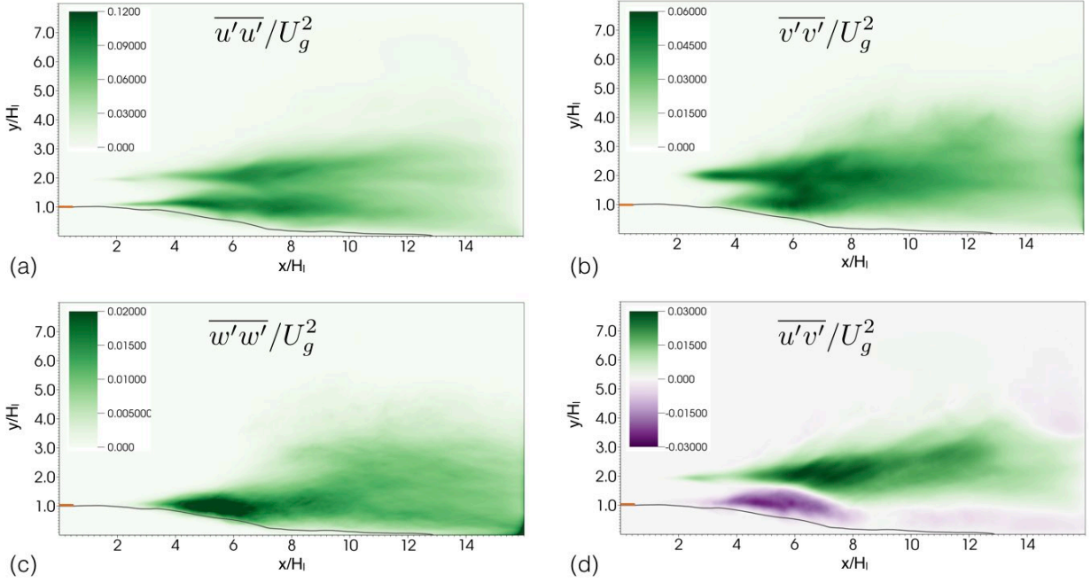
FIGURE 6. Reynolds stress tensor divided by density for Reynolds averaging. The black curve corresponds to \bar{c} = 0.5 . The orange rectangle near the inlet represents the separator plate.
