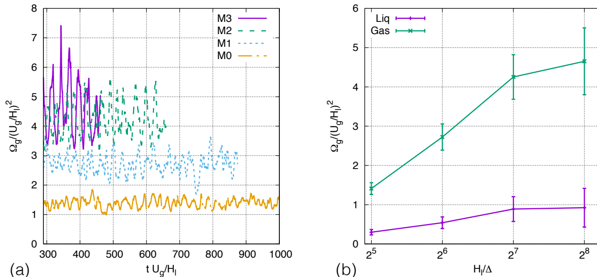
FIGURE 16. (a) Temporal evolution of gas enstrophy of the whole domain and (b) time-averaged liquid and gas enstrophy for different mesh resolutions.
