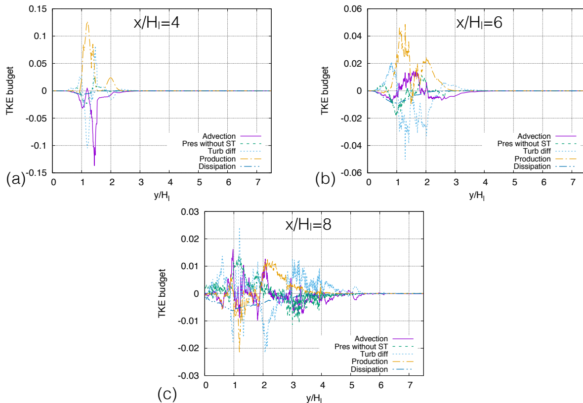
FIGURE 8. Turbulence kinetic energy budget at different streamwise locations. The terms in Eq. (3.19) are normalized by \rho_g U_g^3 / H_l .
