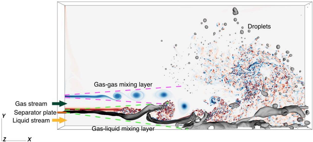
FIGURE 1. A two-phase mixing layer between parallel gas and liquid streams. The grey surface is the liquid-gas interface and the background is the z -component of vorticity.
