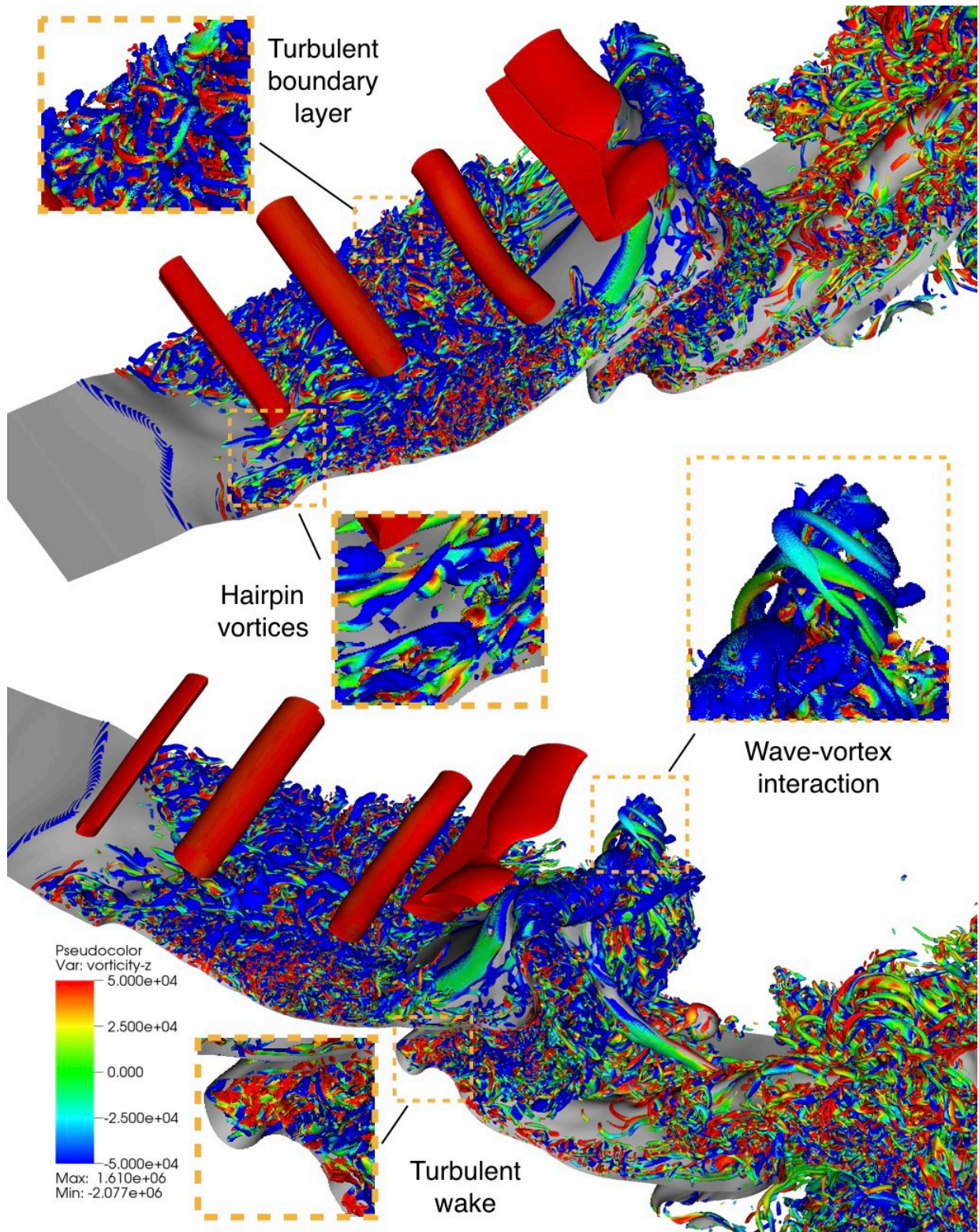
FIGURE 3. A snapshot of the vortical structures near the interface. Vortices are visualized by the \lambda_2 criterion.
