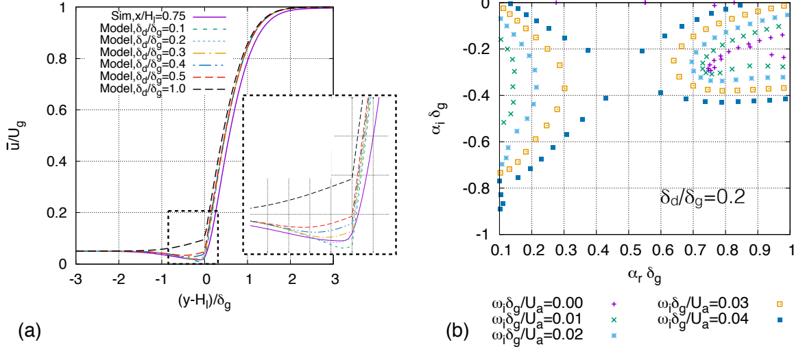
FIGURE 14. Spatio-temporal viscous stability. (a) Models for initial streamwise velocity profile. (b) \omega_i contours to show the pinching point.
