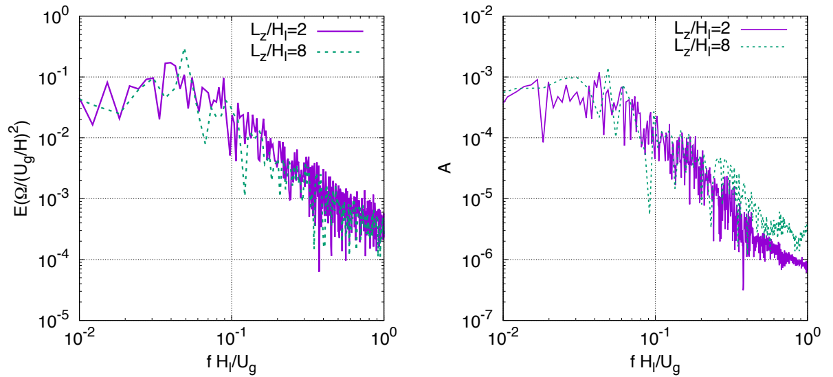
FIGURE 21. Effect of domain width on the spectra of (a) the integrated gas enstrophy in the domain and (b) the interfacial height at x/H_l = 0.75 . L_z/H_l = 2 and 8 for the present and the wider domains.
