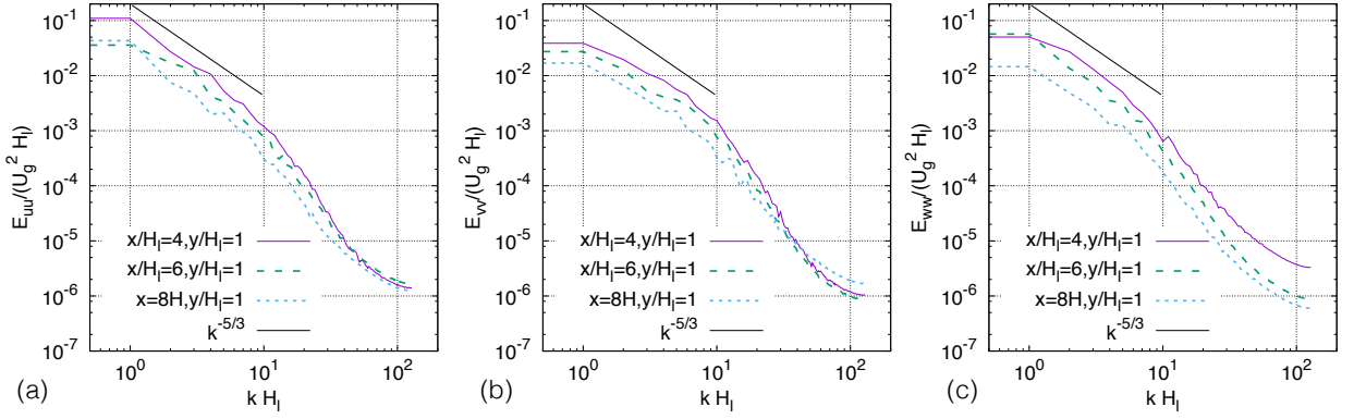
FIGURE 13. Velocity spectra at different streamwise locations.
