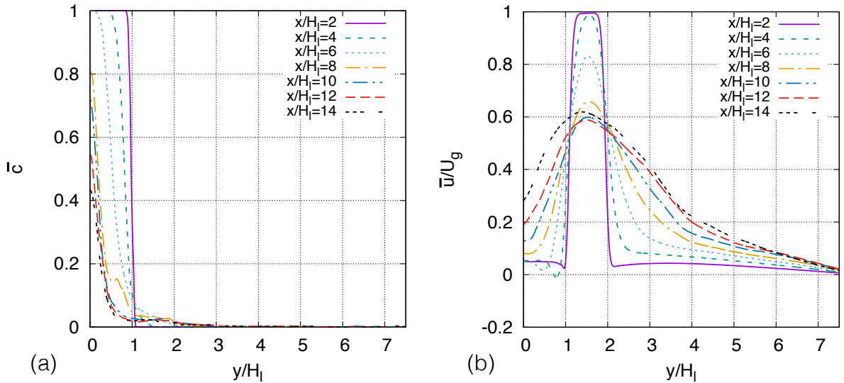
FIGURE 5. Mean flow profiles for Favre averaging at different streamwise locations.
