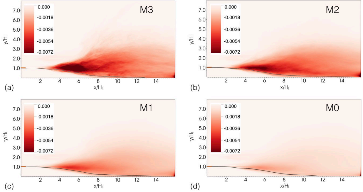
FIGURE 10. Distribution of turbulent kinetic energy dissipation for different mesh resolutions. The black curve corresponds to \bar{c} = 0.5 . The orange rectangle near the inlet represents the separator plate.
