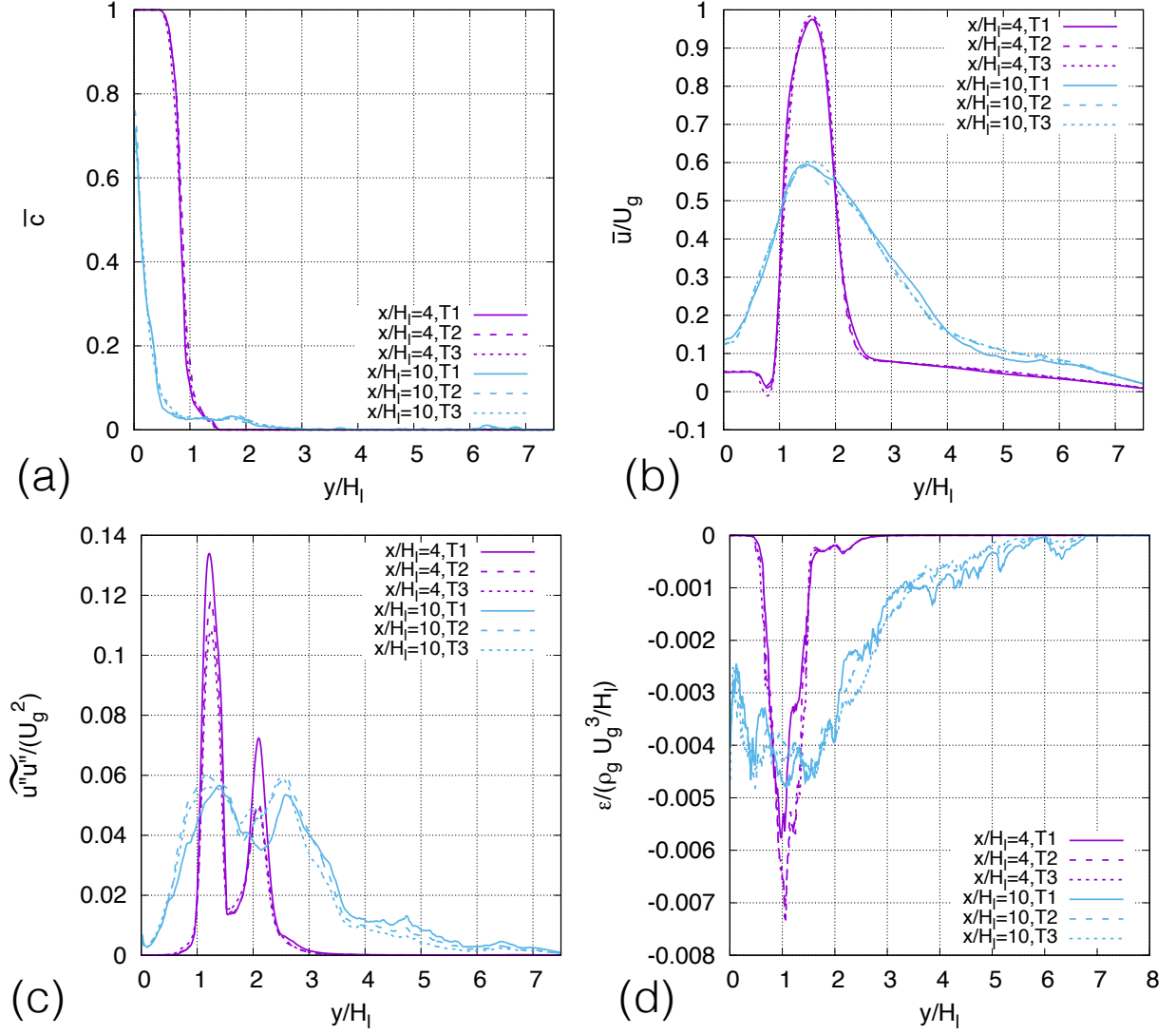
FIGURE 20. Statistical convergence studies for multiphase turbulence statistics.
