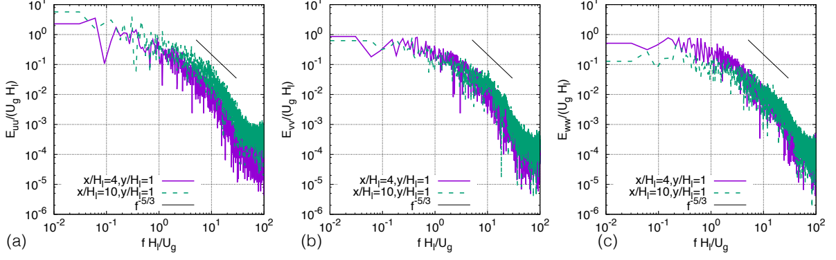
FIGURE 12. Velocity spectra at different locations.
