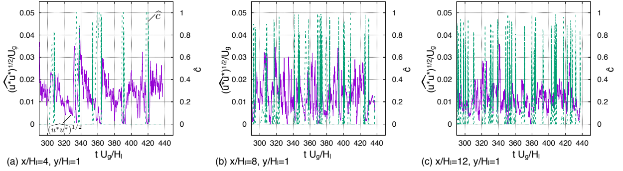
FIGURE 17. Temporal evolution of (\widehat{u^* u^*})^{1/2} (purple solid lines) and \widehat{c} (green dashed lines) at different streamwise locations.
