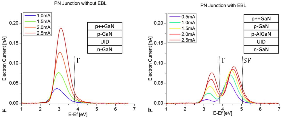
Figure 3: a) EDCs from p-i-n device with a single peak ( \Gamma ) with a high energy threshold \sim 3.7 eV. b) EDCs from p-i-n + \text{EBL} device with two peaks ( \Gamma and SV).
