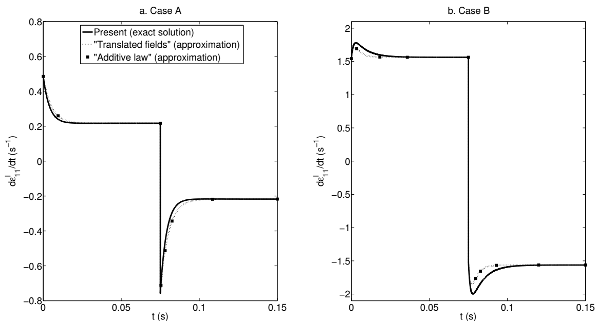
Fig. 6 Time evolution of axial strain rate \dot{\varepsilon}_{11}^I in the inclusion along the tension-compression axis predicted by the present linear homogenization Mori-Tanaka approach based on the exact interaction law for the Eshelby's inclusion problem (Eqs. 32 to 41) in the “case A” (a) and in the “case B” (b). For both cases, the present model (solid lines) matches exactly the inverse Laplace-Carson solutions reported in [15]. For comparisons, the time evolutions of \dot{\varepsilon}_{11}^I given by the approximate “translated fields” method (dashed lines) and “additive interaction” law (points) are reported.
