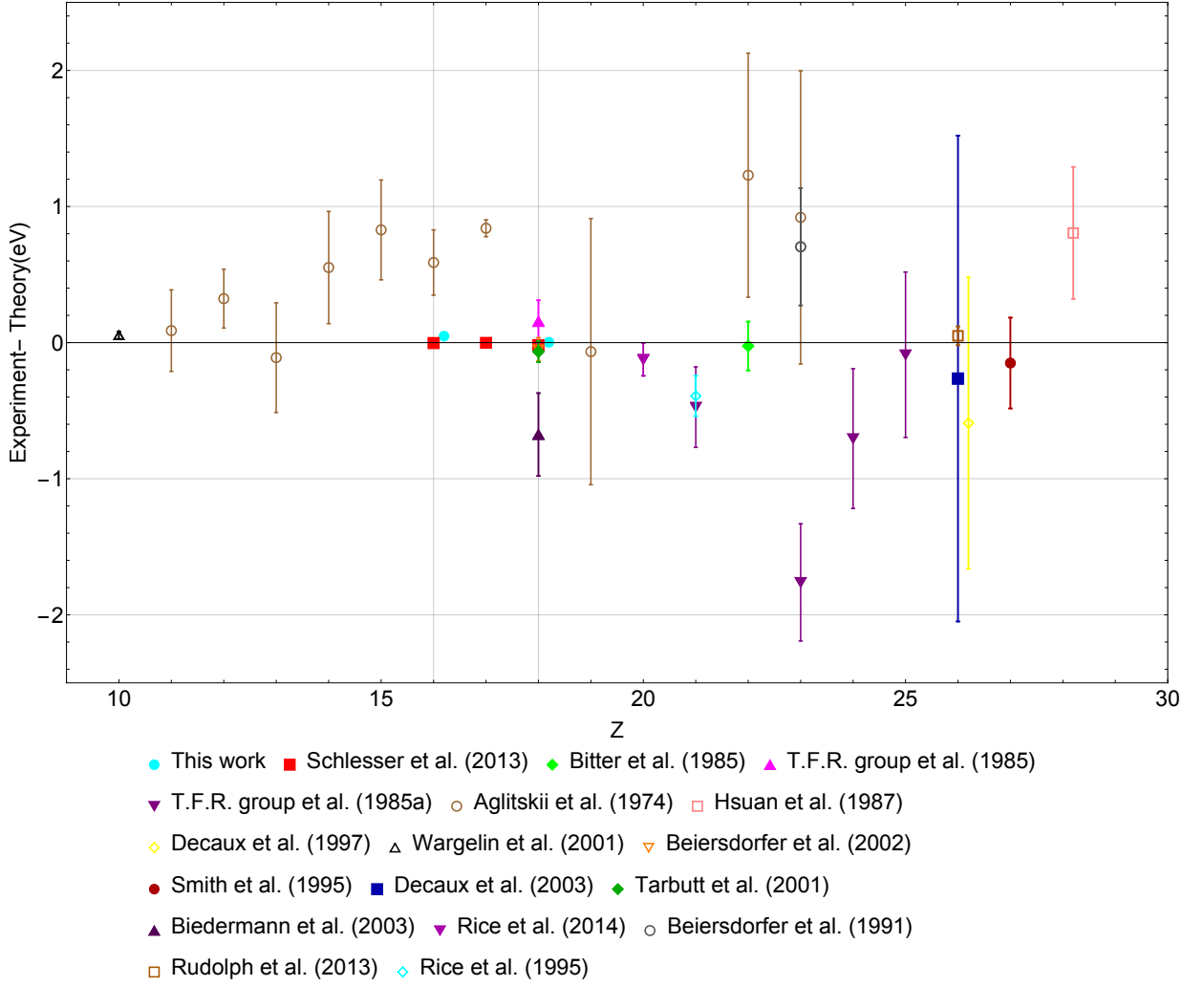
FIG. 12: (Color online) Comparison between Theory [31, 32, 114] and Experiment for the 1s\ 2s\ 2p\ ^2P_{1/2} \rightarrow 1s^2\ 2s^2\ S_{1/2} transition. Experimental values from: Schlessler et al. (2013)[51], Bitter et al. (1985)[36], T.F.R. group et al. (1985)[37], T.F.R. group et al. (1985a)[38], Aglitskii et al. (1974)[34], Hsuan et al. (1987)[39], Decaux et al. (1997)[44], Wargelin et al. (2001)[45], Beiersdorfer et al. (2002)[47], Smith et al. (1995)[42], Decaux et al. (2003)[48], Tarbutt et al. (2001)[46], Biedermann et al. (2003)[49], Rice et al. (2014)[52], Beiersdorfer et al. (1991)[40], Rudolph et al. (2013)[50], Rice et al. (1995)[43].
