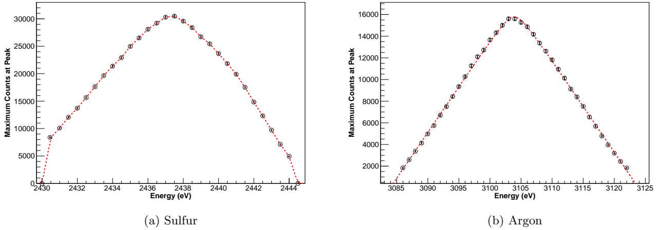
FIG. 16: (Color online) Transmitted intensity by the spectrometer for Li-like sulfur and argon as a function of x-ray energy following [126]. The red curve represents a fit with splines in sulfur and the fit with Eq. (4) in argon.
