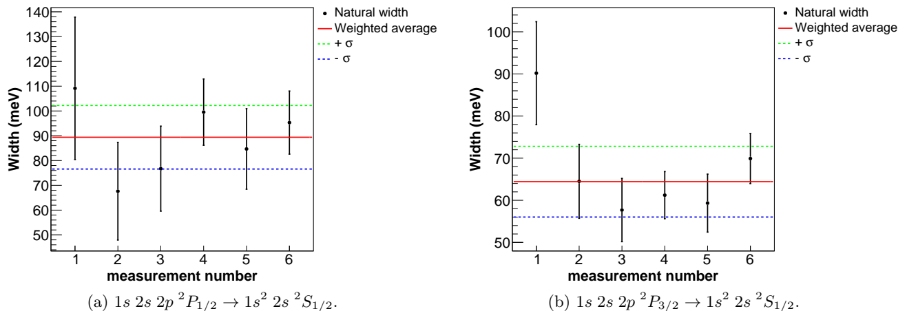
FIG. 4: (Color online) Natural widths of all spectra recorded during the measurement of the 1s\ 2s\ 2p^2 P_J \rightarrow 1s^2\ 2s^2 S_{1/2} , J = 1/2, 3/2 Li-like argon transitions. The weighted average and the 68% confidence interval ( \pm 1\sigma ) are also shown.
