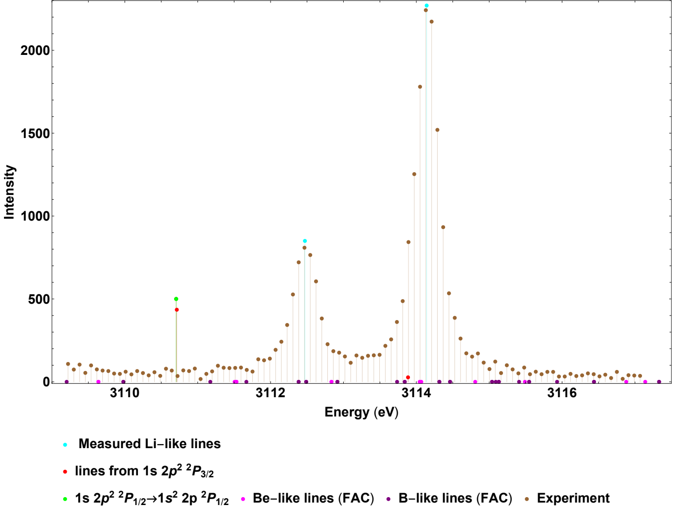
FIG. 18: (Color online) Possible blends to the 1s\ 2s\ 2p\ ^2P_{1/2} \rightarrow 1s^2\ 2s\ 2s\ ^2S_{1/2} and 1s\ 2s\ 2p\ ^2P_{3/2} \rightarrow 1s^2\ 2s\ 2s\ ^2S_{1/2} transitions in argon. The 1s\ 2p^2\ ^2P_{3/2} \rightarrow 1s^2\ 2p^2\ ^2P_{3/2} , 1s\ 2p^2\ ^2P_{3/2} \rightarrow 1s^2\ 2p^2\ ^2P_{1/2} and the 1s\ 2p^2\ ^2P_{1/2} \rightarrow 1s^2\ 2p^2\ ^2P_{1/2} transition energies are from Ref. [31]. The relative intensities of the 1s\ 2p^2\ ^2P_{3/2} \rightarrow 1s^2\ 2p^2\ ^2P_{3/2} and 1s\ 2p^2\ ^2P_{3/2} \rightarrow 1s^2\ 2p^2\ ^2P_{1/2} transitions are evaluated using branching ratios calculated with FAC. The absence of a line at the expected position in the experimental spectrum shows that the contribution of this line to the intensity of the 1s\ 2s\ 2p\ ^2P_J \rightarrow 1s^2\ 2s\ 2s\ ^2S_{1/2} doublet is negligible. The energies and relative intensities of the Be-like and B-like lines are also evaluated using FAC. Their contributions are very small.
