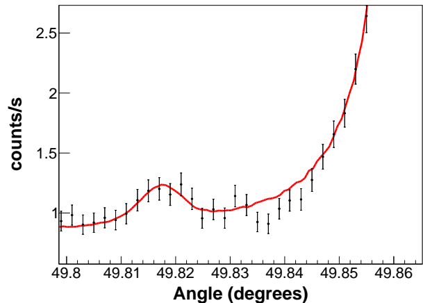
(b) Zoom on 1s\ 2s\ 2p\ ^4P_{5/2} \rightarrow 1s^2\ 2s^2\ ^2S_{1/2} .
