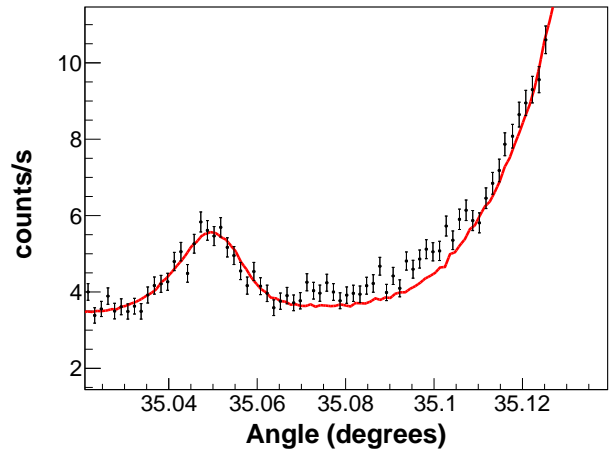
(b) Zoom on 1s\ 2s\ 2p\ ^4P_{5/2} \rightarrow 1s^2\ 2s^2\ ^2S_{1/2} .
