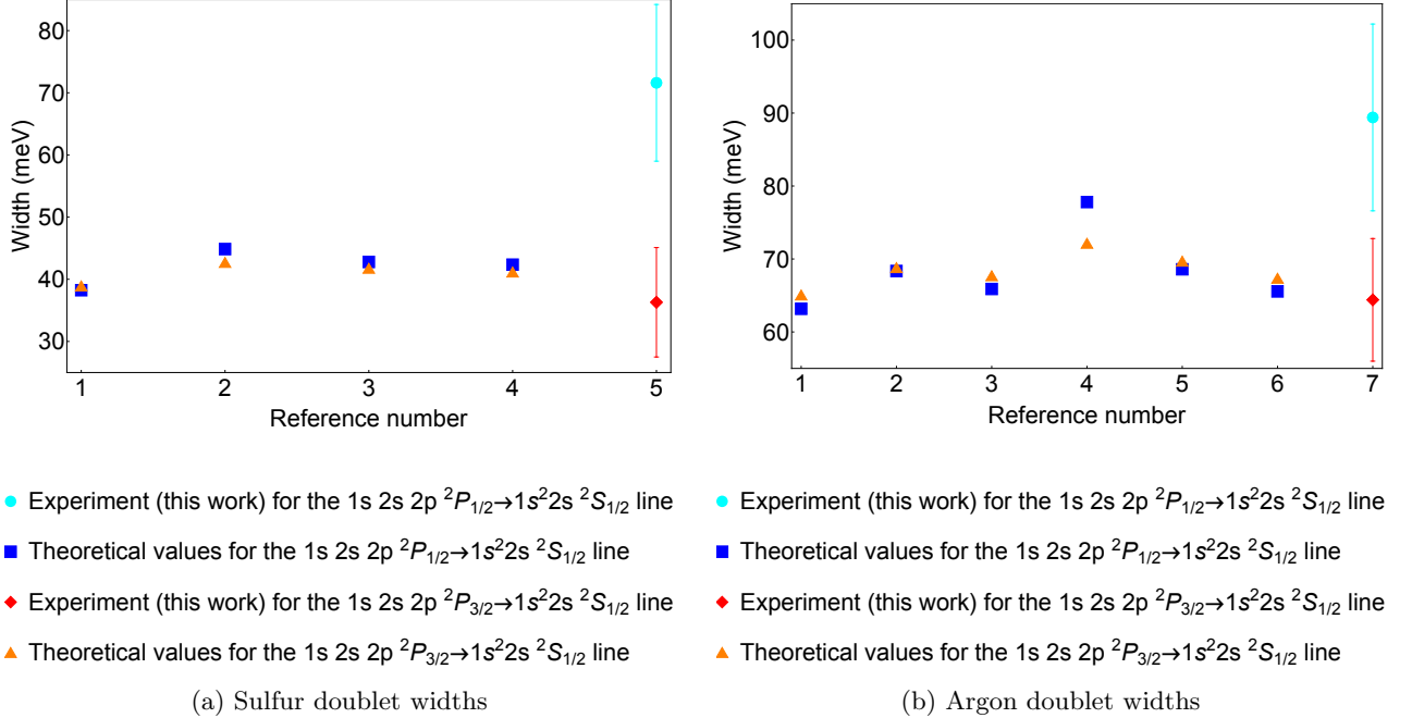
FIG. 11: (Color online) Comparison between the measured and theoretical values for the widths. Sulfur references: 1, This work, MCDF; 2, this work FAC; 3, Ref. [110]; 4, Ref. [111]; 5, this work, experiment. Argon references: 1, This work, MCDF; 2, this work FAC; 3, Ref. [110]; 4, Ref. [112]; 5, Ref. [113]; 6, Ref. [111]; 7, this work, experiment.
