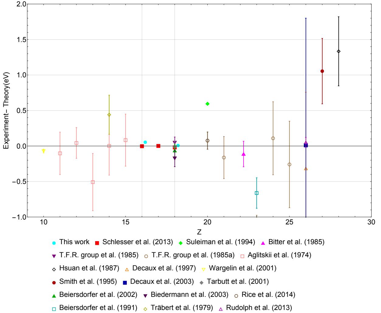
FIG. 13: (Color online) Comparison between theory [31, 32, 114] and all available experiment for the 1s\ 2s\ 2p^2 P_{3/2} \rightarrow 1s^2\ 2s^2 S_{1/2} transition. Experimental values from: Schlessler et al. (2013)[51], Suleiman et al. (1994)[41], Bitter et al. (1985)[36], T.F.R. group et al. (1985)[37], T.F.R. group et al. (1985a)[38], Aglitskii et al. (1974)[34], Hsuan et al. (1987)[39], Decaux et al. (1997)[44], Wargelin et al. (2001)[45], Smith et al. (1995)[42], Decaux et al. (2003)[48], Tarbutt et al. (2001)[46], Beiersdorfer et al. (2002)[47], Biedermann et al. (2003)[49], Rice et al. (2014)[52], Beiersdorfer et al. (1991)[40], Träbert et al. (1979)[35], Rudolph et al. (2013)[50], Rice et al. (1995)[43].
