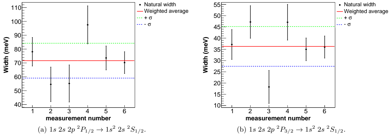
FIG. 3: (Color online) Natural widths of all spectra recorded during the measurement of the 1s\ 2s\ 2p^2\ P_J \rightarrow 1s^2\ 2s^2\ S_{1/2} , J = 1/2, 3/2 Li-like sulfur transitions. The weighted average and the 68% confidence interval ( \pm 1\sigma ) are also shown.
