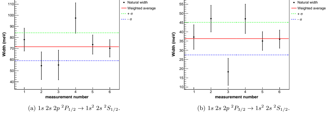
FIG. 5: (Color online) Natural widths of all spectra recorded during the measurement of the 1s\ 2s\ 2p^2\ P_J \rightarrow 1s^2\ 2s^2\ S_{1/2} , J = 1/2, 3/2 Li-like sulfur transitions. The weighted average and the 68% confidence interval ( \pm 1\sigma ) are also shown.
