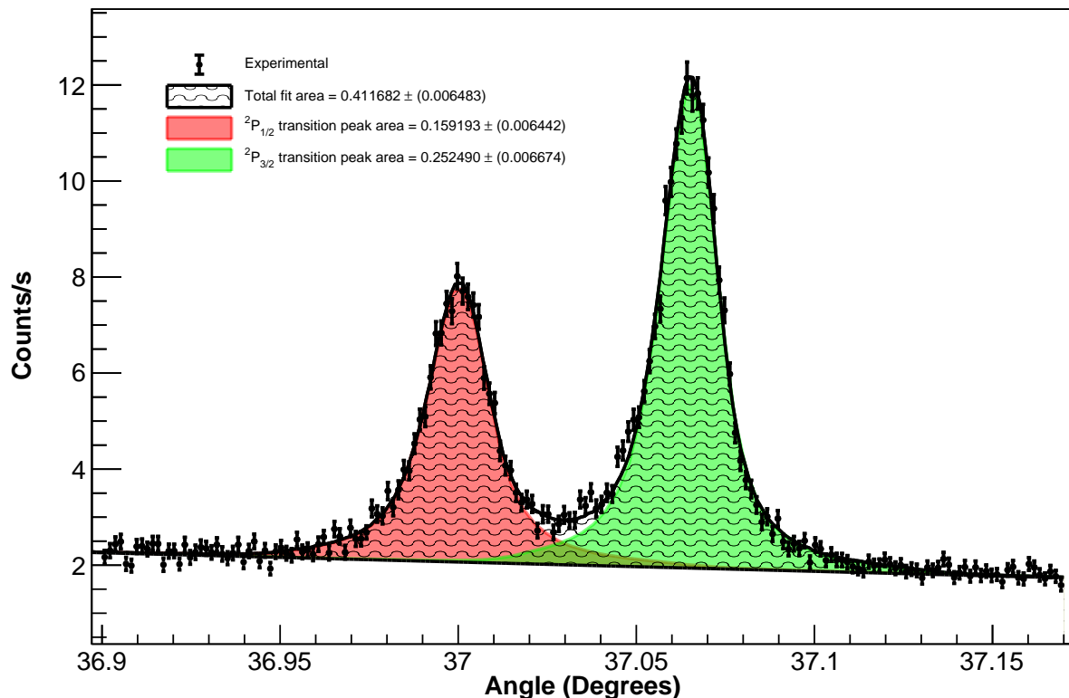
FIG. 15: (Color online) Integral example of the Li-like sulfur 1s\ 2s\ 2p\ ^2P_J \rightarrow 1s^2\ 2s^2\ ^2S_{1/2} , J = 1/2, 3/2 doublet dispersive spectrum. The solid black curve represents the total fit to the spectrum from Eq. (1) with its respective integral represented by the shadowed white area with the wave-like texture. Red ( J = 1/2 ) and green ( J = 3/2 ) solid curves represent the individual fits to each peak while the individual integrals are represented by the shadowed areas with the same color. The values obtained for the integrals with their respective estimated error are presented in the plot legend.
