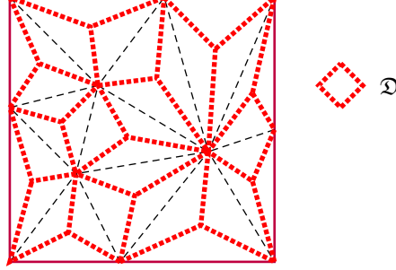
FIGURE 2. An example of diamond mesh \mathcal{D}
