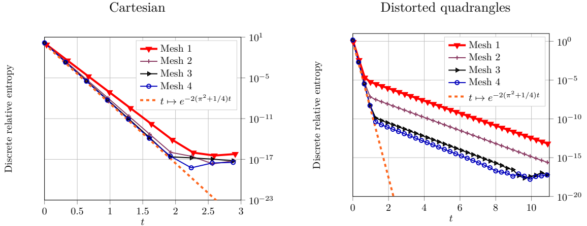
FIGURE 7. DDFV . Exponential decay of the relative entropy on a sequence of Cartesian (left) and quadrangular (right) meshes in the degenerate case \varepsilon = 0 and \Lambda_{11} = 0.1 .
