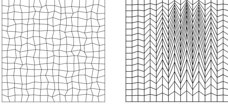
FIGURE 5. DDFV . The distorted quadrangular (left) and Kershaw (right) meshes.
