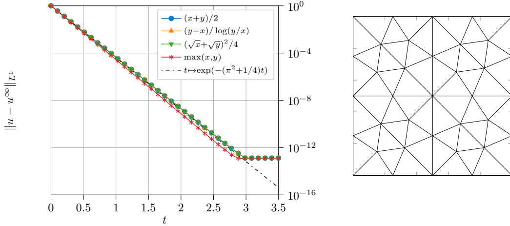
FIGURE 4. TPFA . L^1 distance between the numerical solution and the steady state (left) on the coarsest mesh (right).
