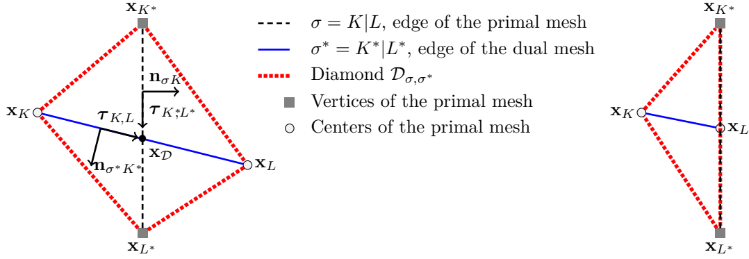
FIGURE 3. Definition of the diamonds \mathcal{D}_{\sigma, \sigma^*} and related notations.
