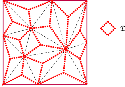
FIGURE 2. An example of diamond mesh \mathcal{D}
