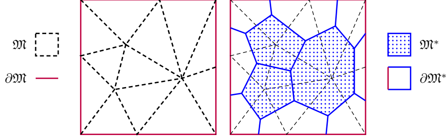
FIGURE 1. An example of primal and dual meshes
