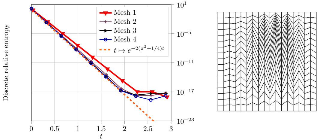
FIGURE 5. DDFV . Exponential decay of the relative entropy (left) on a sequence of Kershaw meshes with the coarsest mesh (right).
