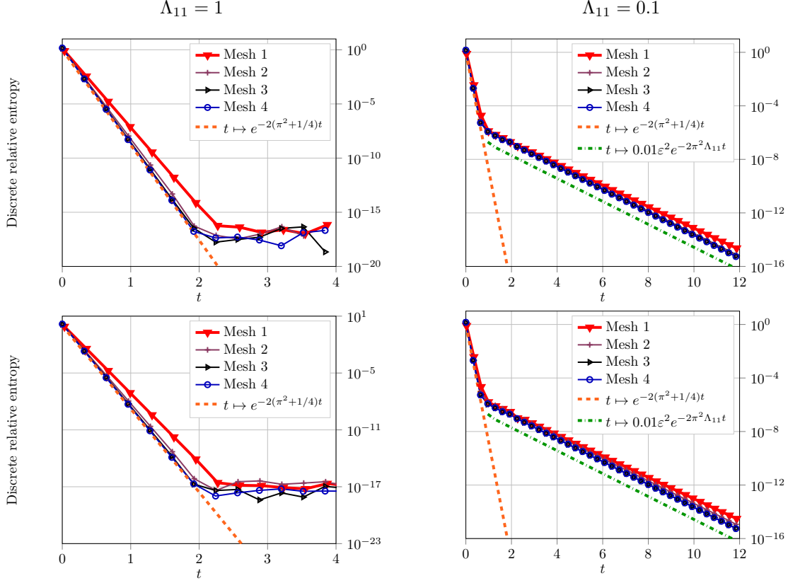
FIGURE 6. DDFV . Exponential decay of the relative entropy on a sequence of Cartesian (top row) and quadrangular (bottom row) meshes mesh with \epsilon = 10^{-2} and \Lambda_{11} = 1 (left column) or \Lambda_{11} = 0.1 (right column).
