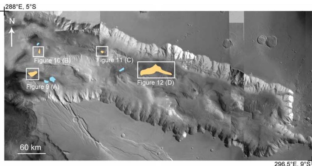
Figure 5. Location map of spectral signatures in East Candor Chasma ( 63.5^{\circ}\text{W} – 72^{\circ}\text{W} , 5^{\circ}\text{S} – 9^{\circ}\text{S} ), superimposed on a mosaic of HRSC images. The three analysis methods used in this study take distinct spectral properties into account. This multimethod approach improves the detection confidence. Sites with robust detections are indicated in orange, sites where the detection of ferric oxides still has to be confirmed are indicated in blue. Locations of Figures 9, 10, 11, and 12 (corresponding to sites A, B, C, and D respectively) are indicated.
