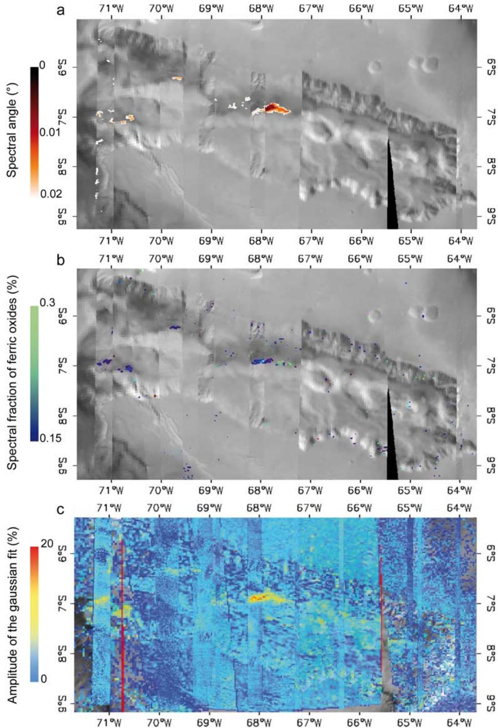
Figure 3. Distribution maps of ferric oxides in East Candor Chasma ( 63.5^{\circ}\text{W} – 72^{\circ}\text{W} , 5^{\circ}\text{S} – 9^{\circ}\text{S} ) obtained with three methods of analysis of OMEGA data. (a) Spectral Angle Mapper. Spectral angle (in degree) between OMEGA spectra and the end-member with spectral characteristics of ferric oxides shown on Figure 2. Colored areas represent the regions with a high spectral similarity with this end-member (spectral angle \leq 0.02^{\circ} ). (b) Spectral Mixing Analysis. Colors represent the mixing coefficient of ferric oxide in the overall spectrum. It is not absolute mineral proportion. (c) Amplitude of the MGM Gaussian fit to the ferric oxide absorption band centered at 0.9\ \mu\text{m} . The deeper the Gaussian, the stronger the spectral signature is.
