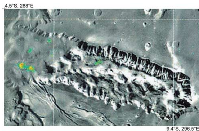
Figure 8. Distribution of gray crystalline hematite detected by TES in East Candor Chasma [ Christensen et al. , 2001].
