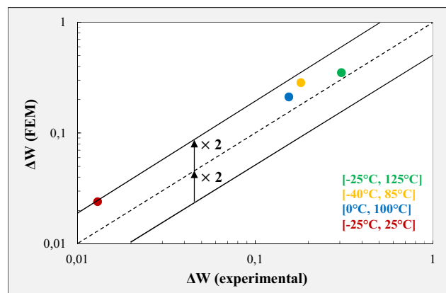
Figure 12. Experimental and numerical strain energy densities for each thermal cycling condition
